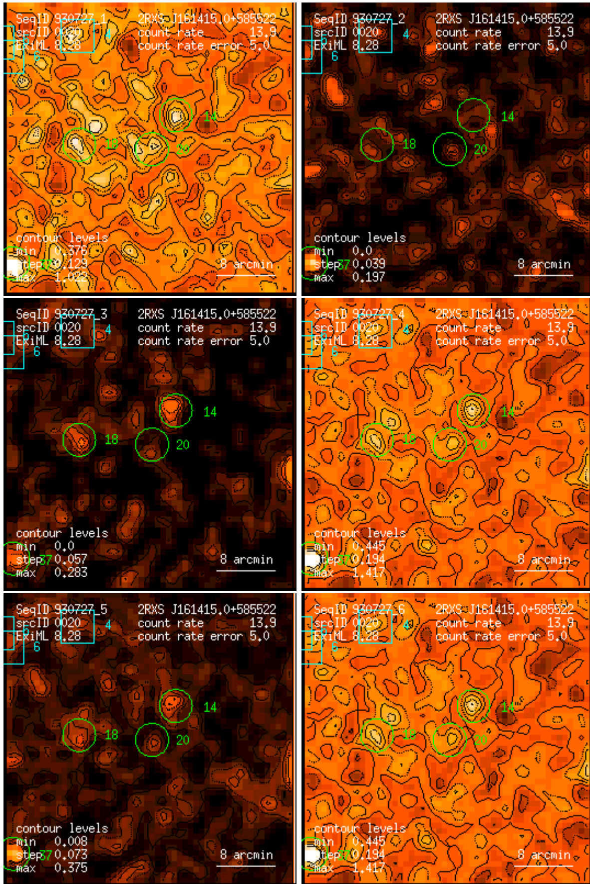
Figure 20: RASS 930727: detection 0020: band rate images, Gaussian filter: (1) PSPC channels 11 – 41, (2) 52 – 90, (3) 91 – 201, (4) 11 – 235, (5) 52 – 201, (6) 11 – 201. Broad band rates in counts/ks. Band rate contour levels in counts/ks/arcmin 2 .
