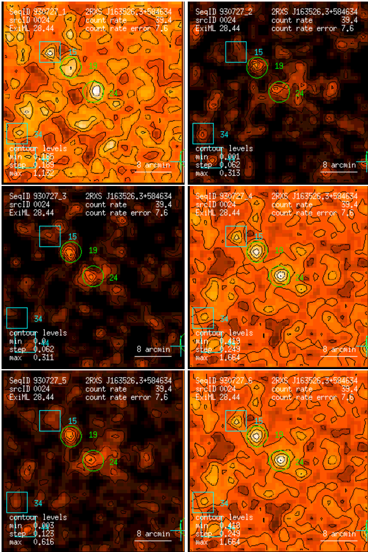
Figure 24: RASS 930727: detection 0024: band rate images, Gaussian filter: (1) PSPC channels 11 – 41, (2) 52 – 90, (3) 91 – 201, (4) 11 – 235, (5) 52 – 201, (6) 11 – 201. Broad band rates in counts/ks. Band rate contour levels in counts/ks/arcmin 2 .
