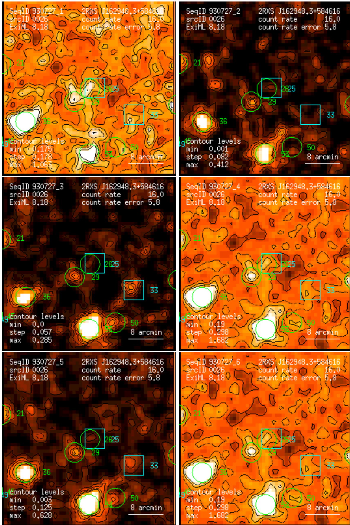
Figure 26: RASS 930727: detection 0026: band rate images, Gaussian filter: (1) PSPC channels 11 – 41, (2) 52 – 90, (3) 91 – 201, (4) 11 – 235, (5) 52 – 201, (6) 11 – 201. Broad band rates in counts/ks. Band rate contour levels in counts/ks/arcmin 2 .
