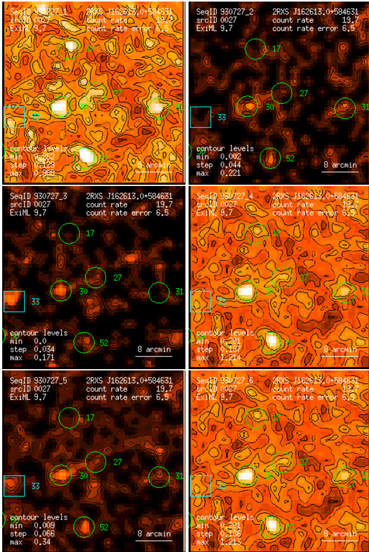
Figure 27: RASS 930727: detection 0027: band rate images, Gaussian filter: (1) PSPC channels 11 – 41, (2) 52 – 90, (3) 91 – 201, (4) 11 – 235, (5) 52 – 201, (6) 11 – 201. Broad band rates in counts/ks. Band rate contour levels in counts/ks/arcmin 2 .
