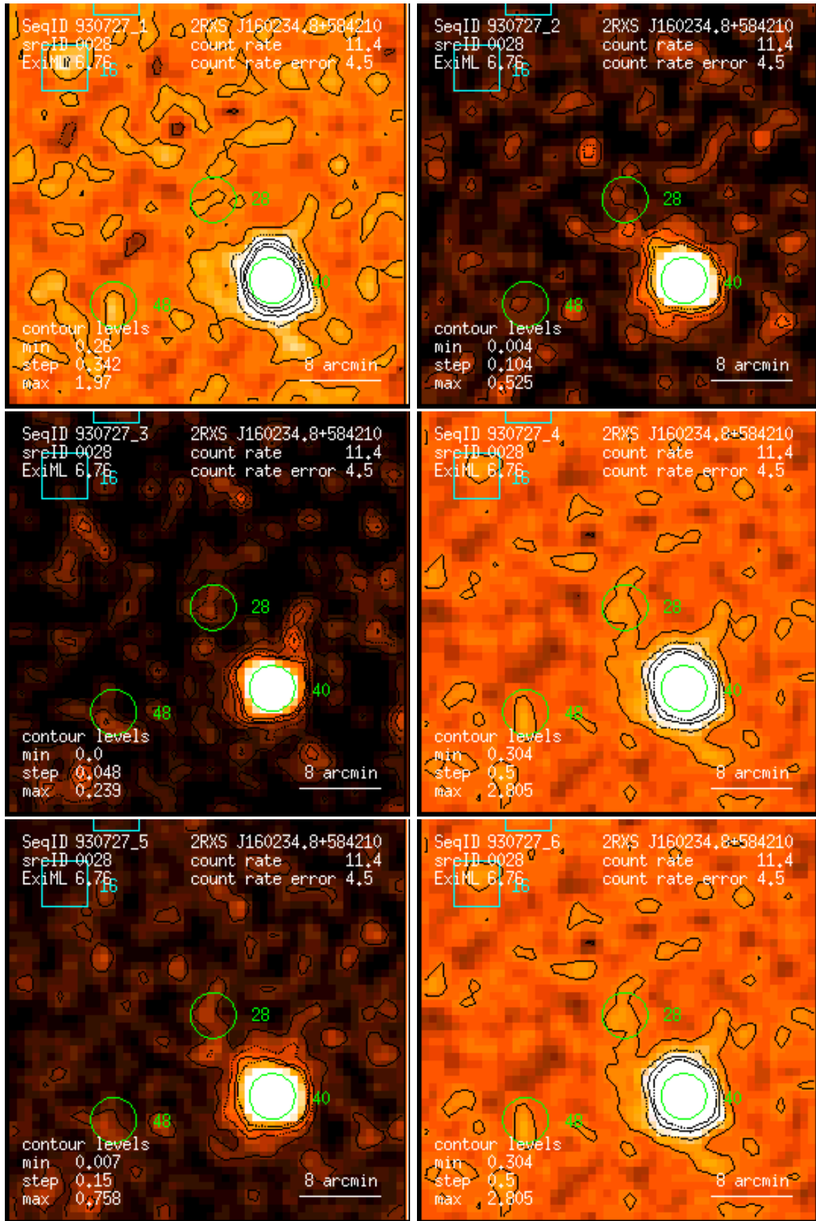
Figure 28: RASS 930727: detection 0028: band rate images, Gaussian filter: (1) PSPC channels 11 – 41, (2) 52 – 90, (3) 91 – 201, (4) 11 – 235, (5) 52 – 201, (6) 11 – 201. Broad band rates in counts/ks. Band rate contour levels in counts/ks/arcmin 2 .
