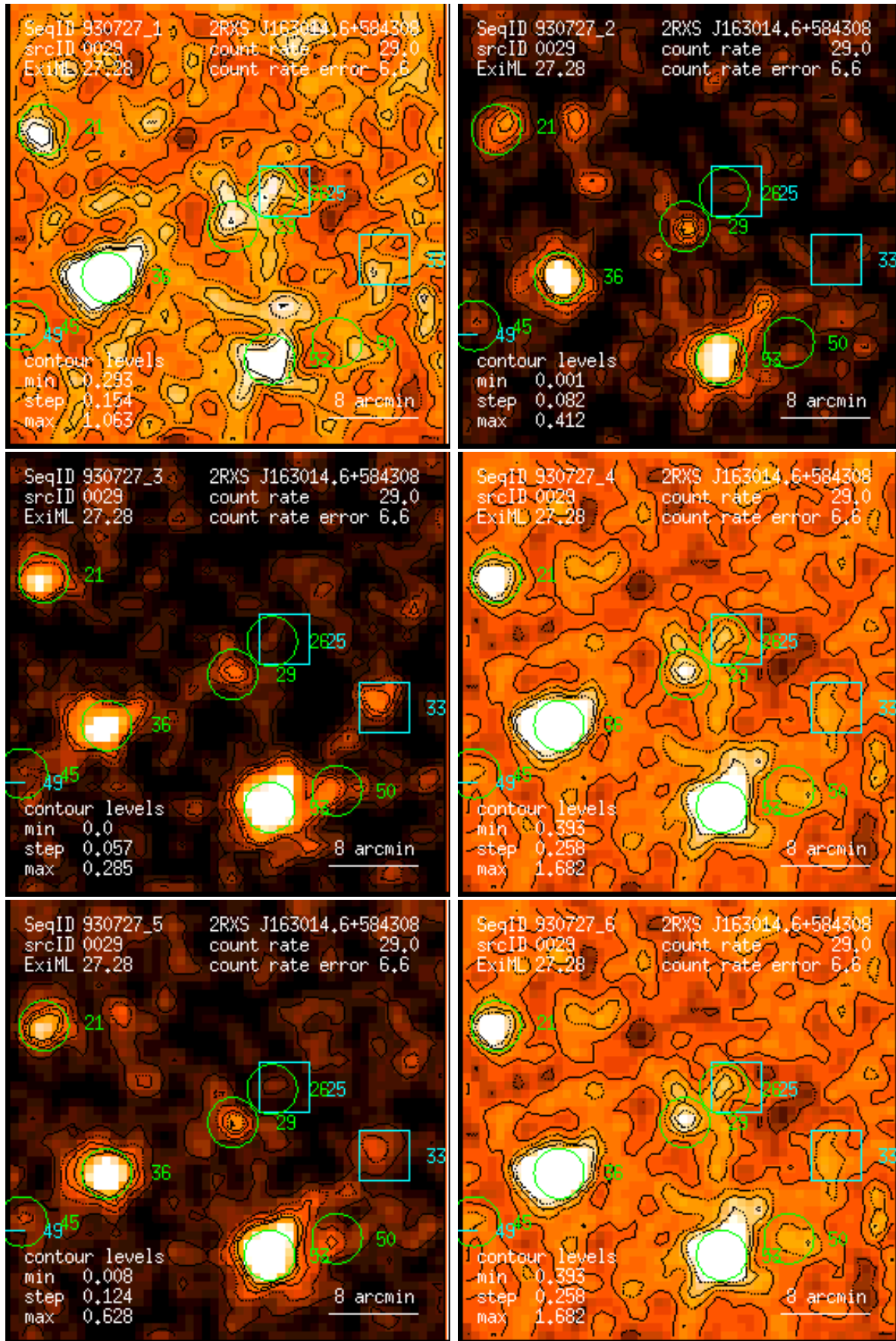
Figure 29: RASS 930727: detection 0029: band rate images, Gaussian filter: (1) PSPC channels 11 – 41, (2) 52 – 90, (3) 91 – 201, (4) 11 – 235, (5) 52 – 201, (6) 11 – 201. Broad band rates in counts/ks. Band rate contour levels in counts/ks/arcmin 2 .
