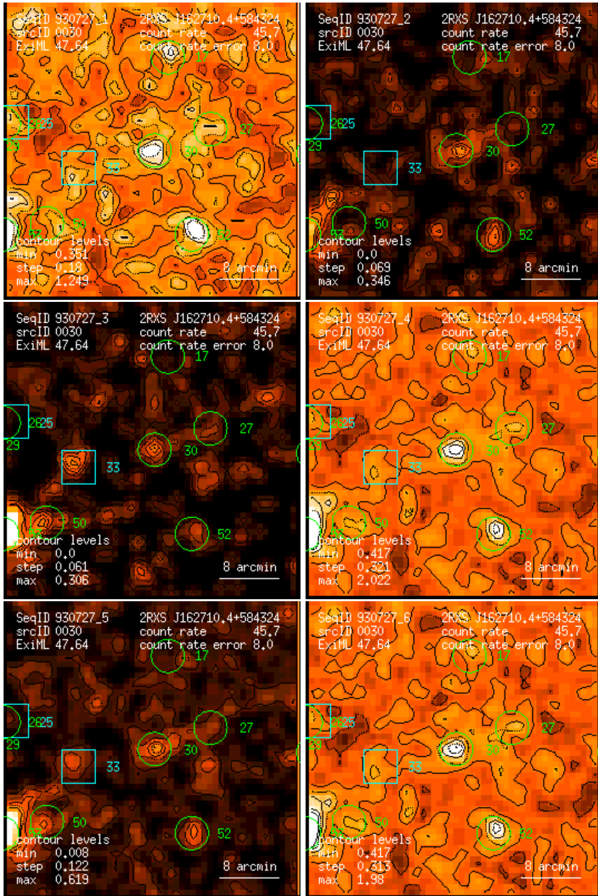
Figure 30: RASS 930727: detection 0030: band rate images, Gaussian filter: (1) PSPC channels 11 – 41, (2) 52 – 90, (3) 91 – 201, (4) 11 – 235, (5) 52 – 201, (6) 11 – 201. Broad band rates in counts/ks. Band rate contour levels in counts/ks/arcmin 2 .
