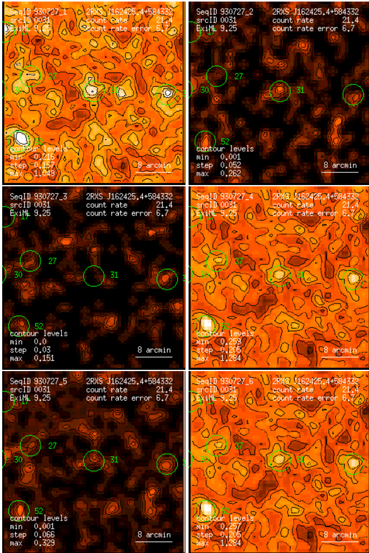
Figure 31: RASS 930727: detection 0031: band rate images, Gaussian filter: (1) PSPC channels 11 – 41, (2) 52 – 90, (3) 91 – 201, (4) 11 – 235, (5) 52 – 201, (6) 11 – 201. Broad band rates in counts/ks. Band rate contour levels in counts/ks/arcmin 2 .
