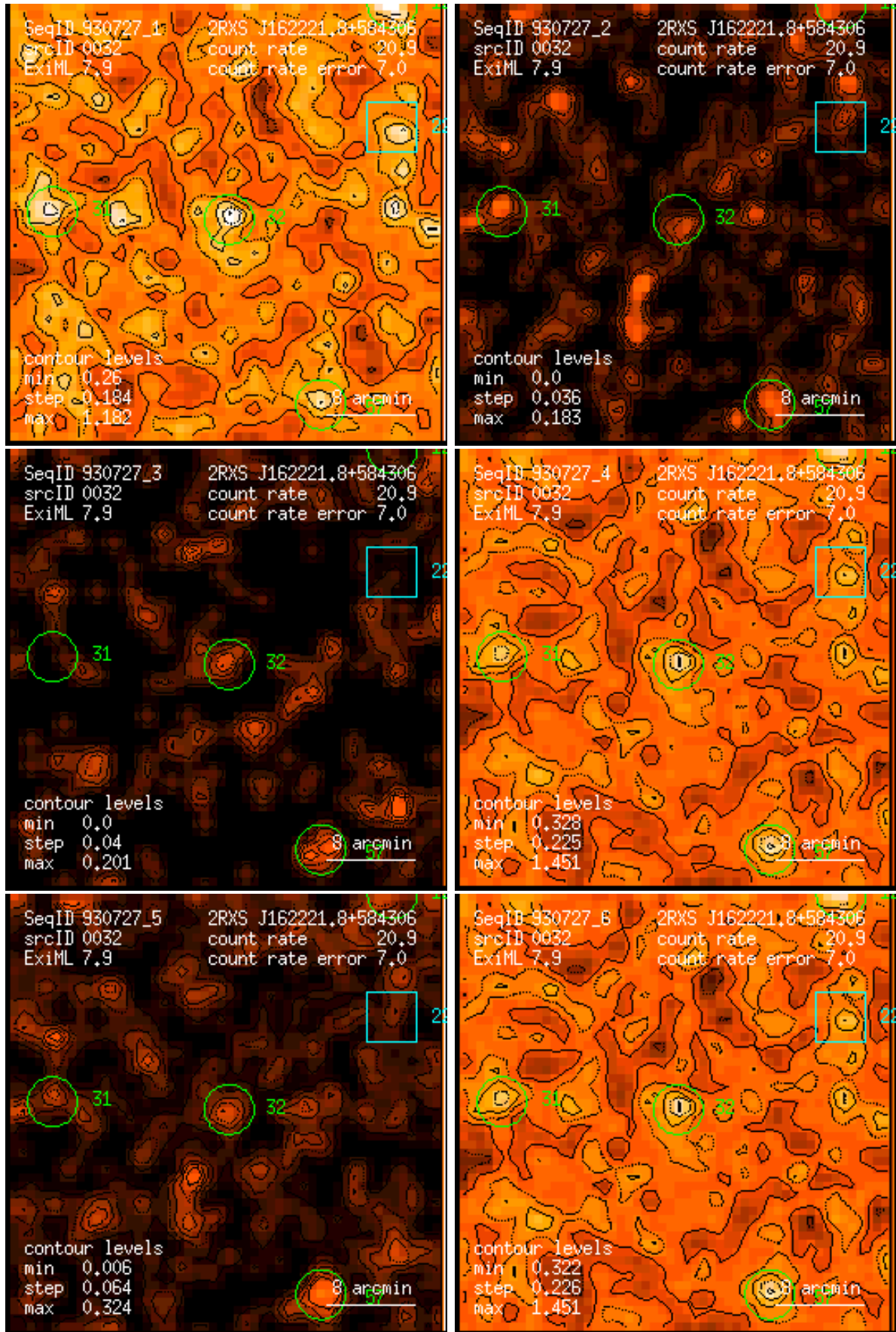
Figure 32: RASS 930727: detection 0032: band rate images, Gaussian filter: (1) PSPC channels 11 – 41, (2) 52 – 90, (3) 91 – 201, (4) 11 – 235, (5) 52 – 201, (6) 11 – 201. Broad band rates in counts/ks. Band rate contour levels in counts/ks/arcmin 2 .
