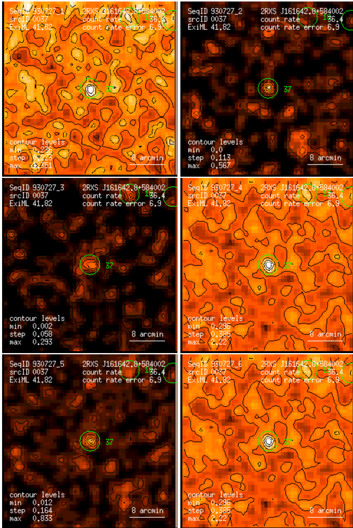
Figure 37: RASS 930727: detection 0037: band rate images, Gaussian filter: (1) PSPC channels 11 – 41, (2) 52 – 90, (3) 91 – 201, (4) 11 – 235, (5) 52 – 201, (6) 11 – 201. Broad band rates in counts/ks. Band rate contour levels in counts/ks/arcmin 2 .
