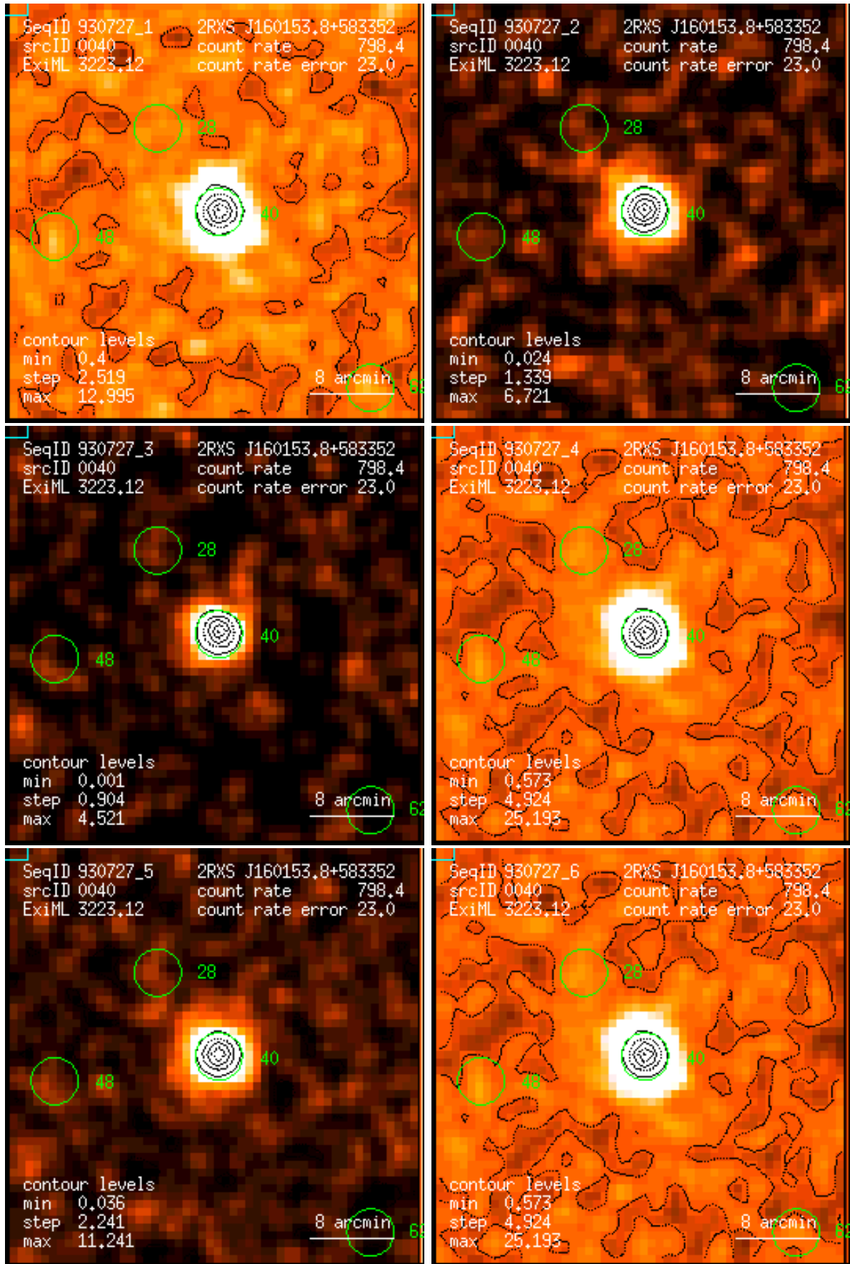
Figure 40: RASS 930727: detection 0040: band rate images, Gaussian filter: (1) PSPC channels 11 – 41, (2) 52 – 90, (3) 91 – 201, (4) 11 – 235, (5) 52 – 201, (6) 11 – 201. Broad band rates in counts/ks. Band rate contour levels in counts/ks/arcmin 2 .
