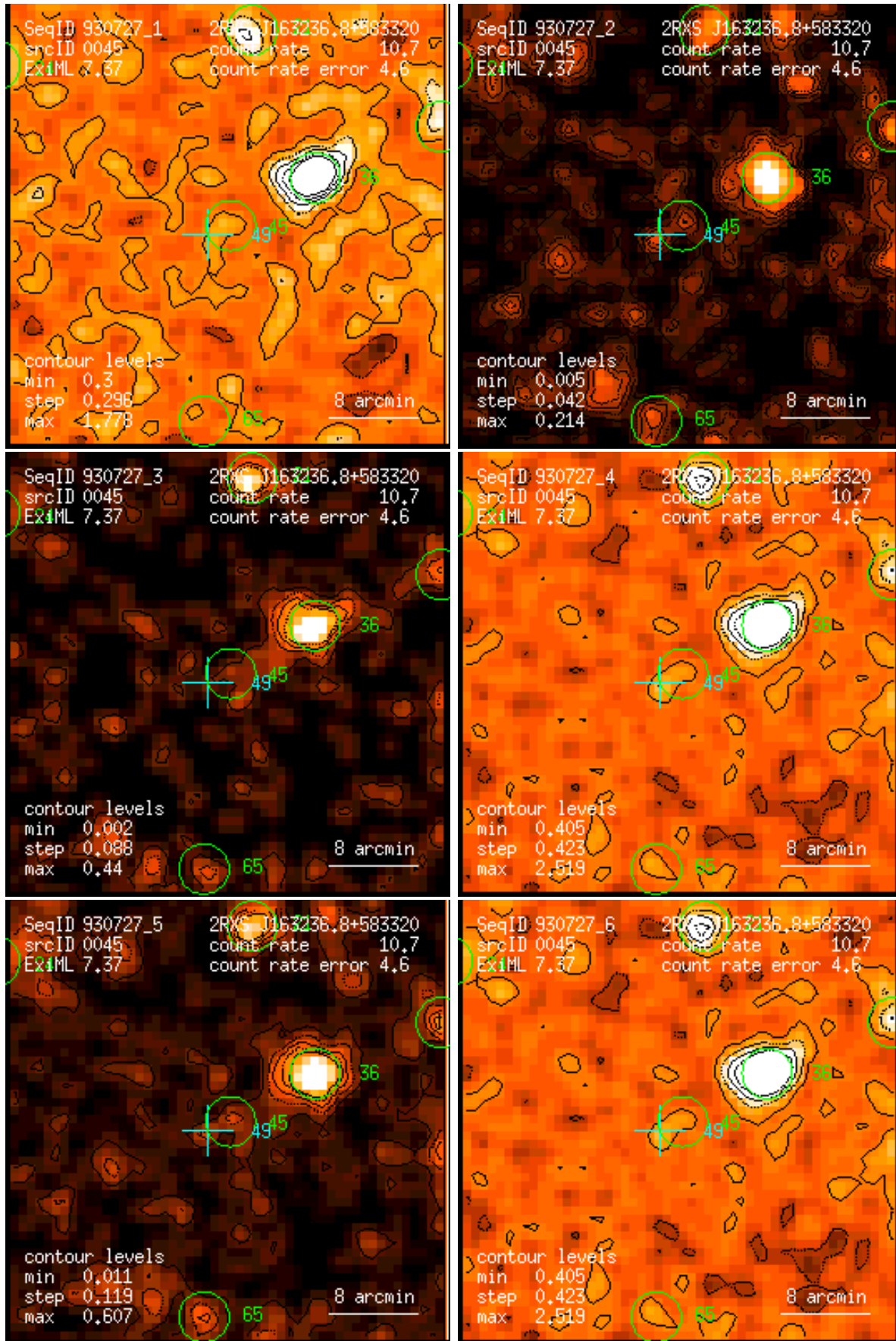
Figure 45: RASS 930727: detection 0045: band rate images, Gaussian filter: (1) PSPC channels 11 – 41, (2) 52 – 90, (3) 91 – 201, (4) 11 – 235, (5) 52 – 201, (6) 11 – 201. Broad band rates in counts/ks. Band rate contour levels in counts/ks/arcmin 2 .
