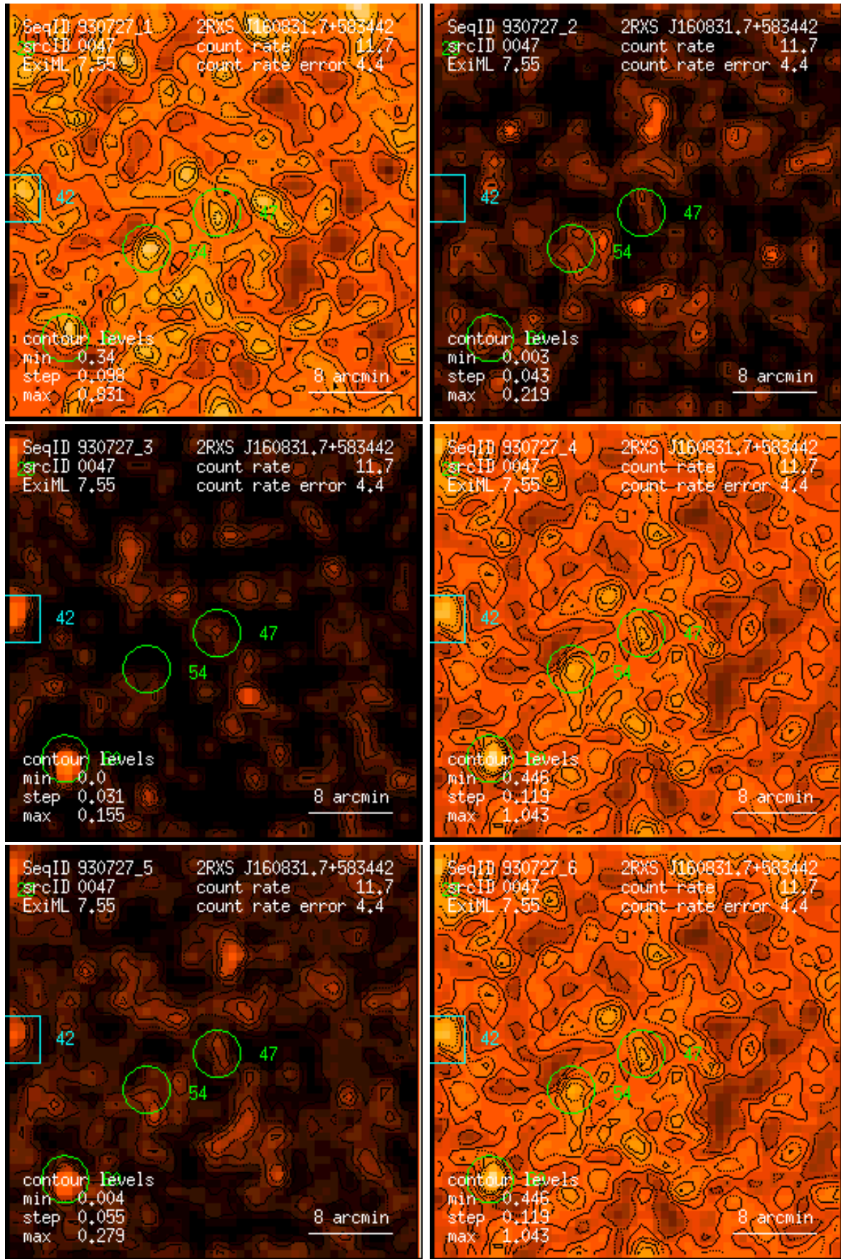
Figure 47: RASS 930727: detection 0047: band rate images, Gaussian filter: (1) PSPC channels 11 – 41, (2) 52 – 90, (3) 91 – 201, (4) 11 – 235, (5) 52 – 201, (6) 11 – 201. Broad band rates in counts/ks. Band rate contour levels in counts/ks/arcmin 2 .
