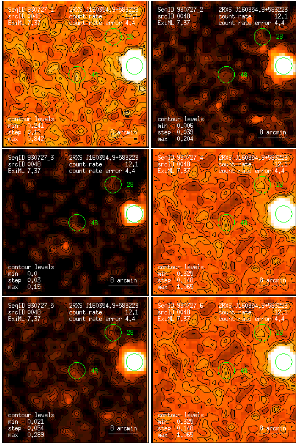
Figure 48: RASS 930727: detection 0048: band rate images, Gaussian filter: (1) PSPC channels 11 – 41, (2) 52 – 90, (3) 91 – 201, (4) 11 – 235, (5) 52 – 201, (6) 11 – 201. Broad band rates in counts/ks. Band rate contour levels in counts/ks/arcmin 2 .
