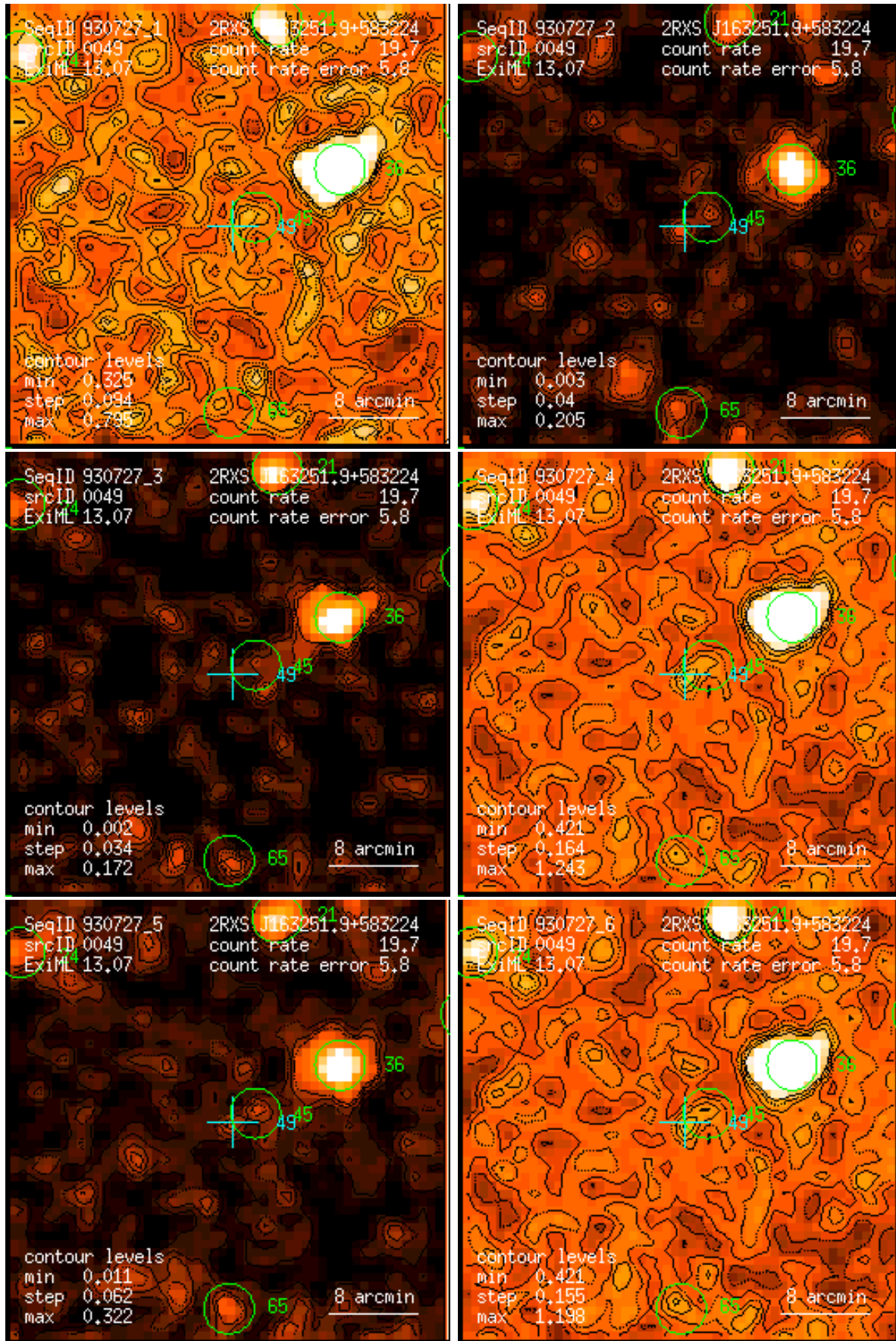
Figure 49: RASS 930727: detection 0049: band rate images, Gaussian filter: (1) PSPC channels 11 – 41, (2) 52 – 90, (3) 91 – 201, (4) 11 – 235, (5) 52 – 201, (6) 11 – 201. Broad band rates in counts/ks. Band rate contour levels in counts/ks/arcmin 2 .
