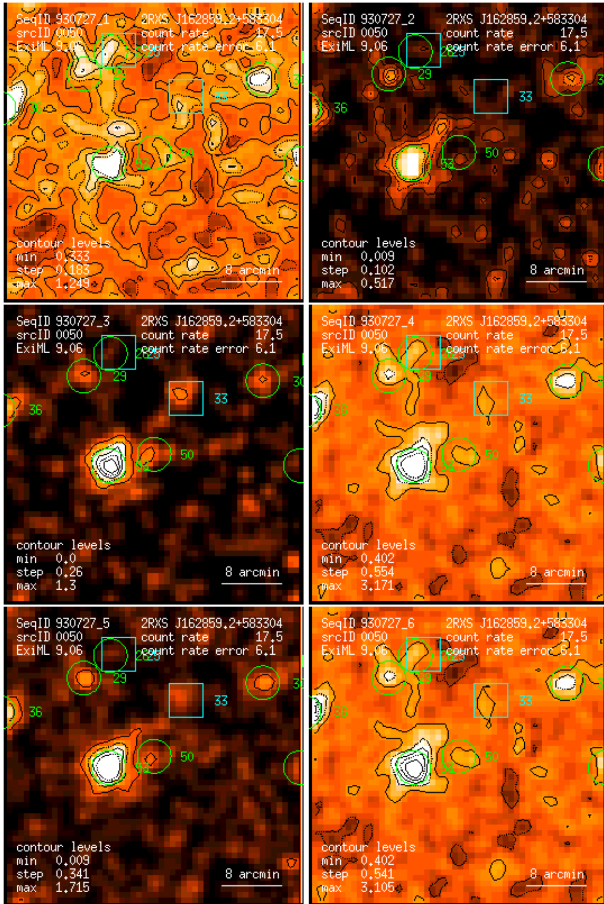
Figure 50: RASS 930727: detection 0050: band rate images, Gaussian filter: (1) PSPC channels 11 – 41, (2) 52 – 90, (3) 91 – 201, (4) 11 – 235, (5) 52 – 201, (6) 11 – 201. Broad band rates in counts/ks. Band rate contour levels in counts/ks/arcmin 2 .
