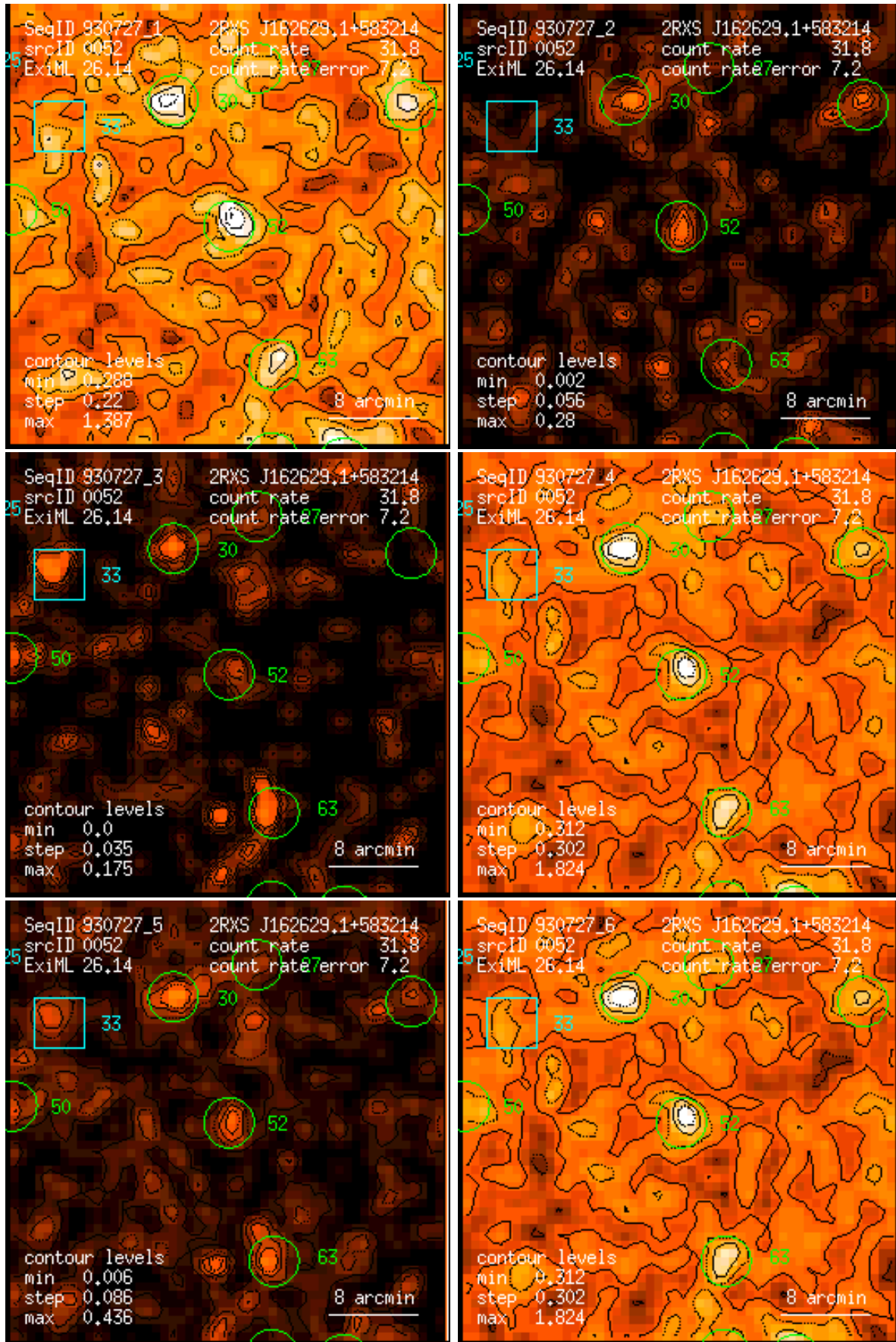
Figure 52: RASS 930727: detection 0052: band rate images, Gaussian filter: (1) PSPC channels 11 – 41, (2) 52 – 90, (3) 91 – 201, (4) 11 – 235, (5) 52 – 201, (6) 11 – 201. Broad band rates in counts/ks. Band rate contour levels in counts/ks/arcmin 2 .
