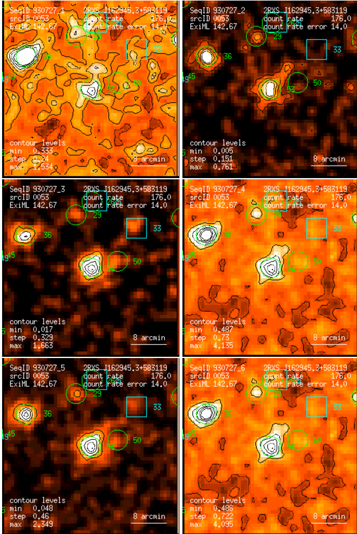
Figure 53: RASS 930727: detection 0053: band rate images, Gaussian filter: (1) PSPC channels 11 – 41, (2) 52 – 90, (3) 91 – 201, (4) 11 – 235, (5) 52 – 201, (6) 11 – 201. Broad band rates in counts/ks. Band rate contour levels in counts/ks/arcmin 2 .
