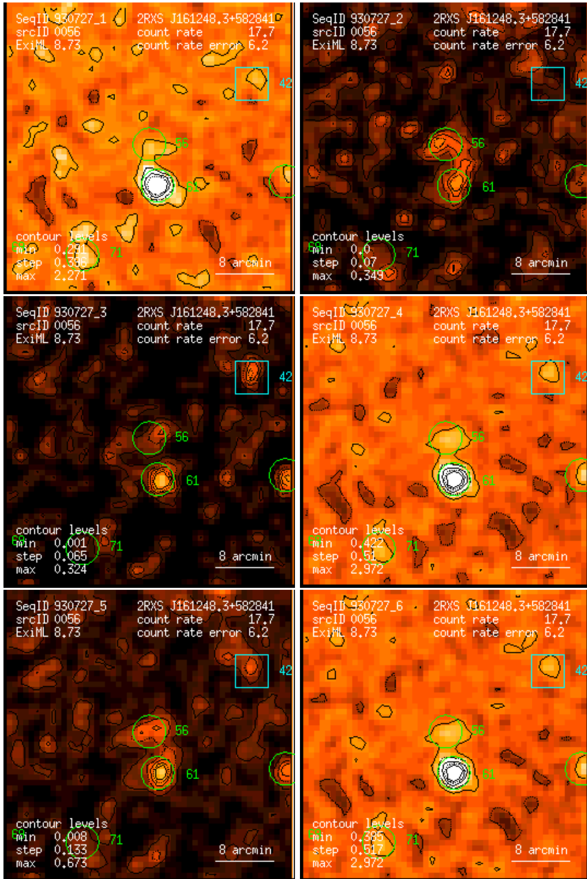
Figure 56: RASS 930727: detection 0056: band rate images, Gaussian filter: (1) PSPC channels 11 – 41, (2) 52 – 90, (3) 91 – 201, (4) 11 – 235, (5) 52 – 201, (6) 11 – 201. Broad band rates in counts/ks. Band rate contour levels in counts/ks/arcmin 2 .
