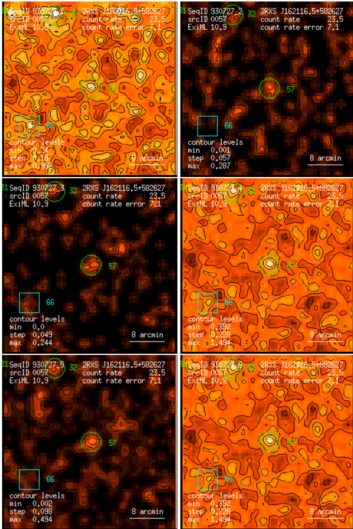
Figure 57: RASS 930727: detection 0057: band rate images, Gaussian filter: (1) PSPC channels 11 – 41, (2) 52 – 90, (3) 91 – 201, (4) 11 – 235, (5) 52 – 201, (6) 11 – 201. Broad band rates in counts/ks. Band rate contour levels in counts/ks/arcmin 2 .
