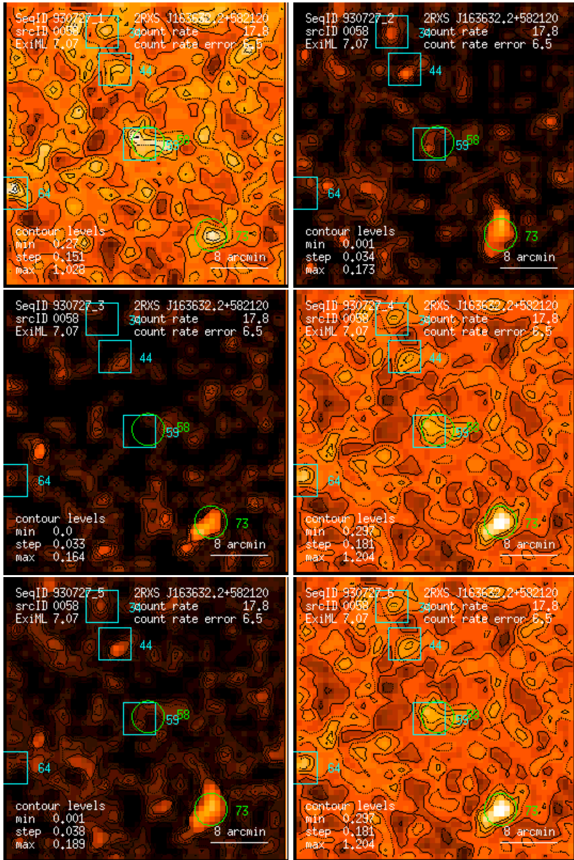
Figure 58: RASS 930727: detection 0058: band rate images, Gaussian filter: (1) PSPC channels 11 – 41, (2) 52 – 90, (3) 91 – 201, (4) 11 – 235, (5) 52 – 201, (6) 11 – 201. Broad band rates in counts/ks. Band rate contour levels in counts/ks/arcmin 2 .
