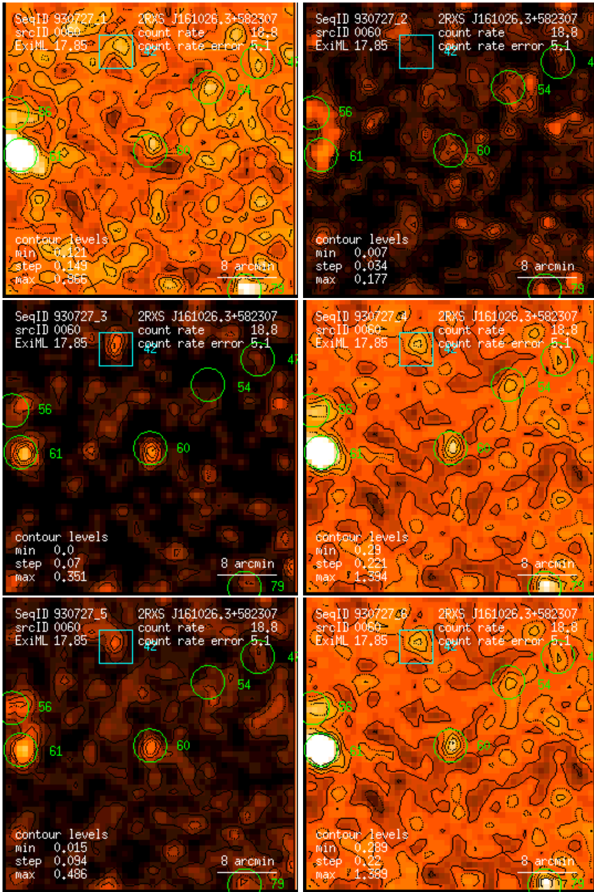
Figure 60: RASS 930727: detection 0060: band rate images, Gaussian filter: (1) PSPC channels 11 – 41, (2) 52 – 90, (3) 91 – 201, (4) 11 – 235, (5) 52 – 201, (6) 11 – 201. Broad band rates in counts/ks. Band rate contour levels in counts/ks/arcmin 2 .
