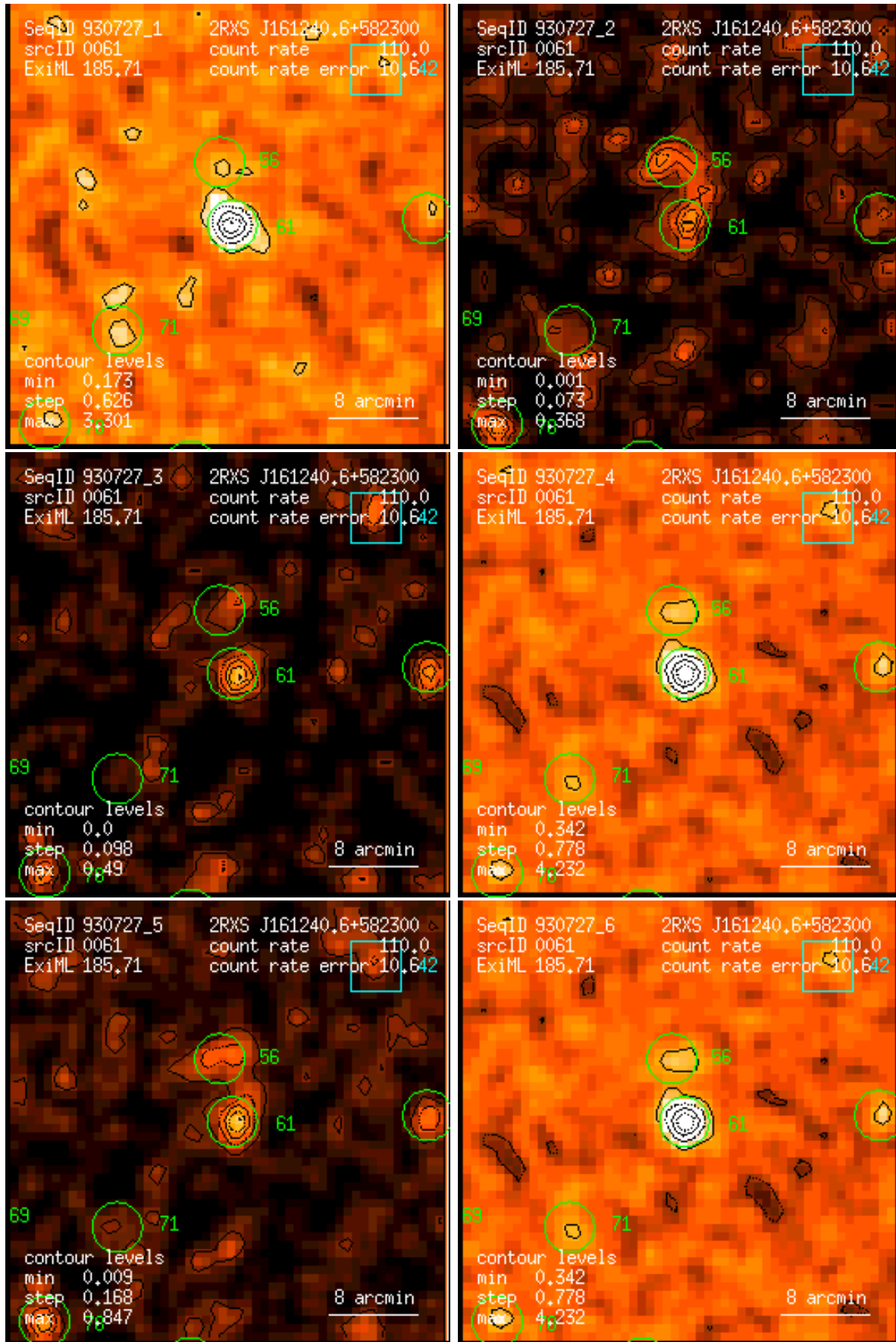
Figure 61: RASS 930727: detection 0061: band rate images, Gaussian filter: (1) PSPC channels 11 – 41, (2) 52 – 90, (3) 91 – 201, (4) 11 – 235, (5) 52 – 201, (6) 11 – 201. Broad band rates in counts/ks. Band rate contour levels in counts/ks/arcmin 2 .
