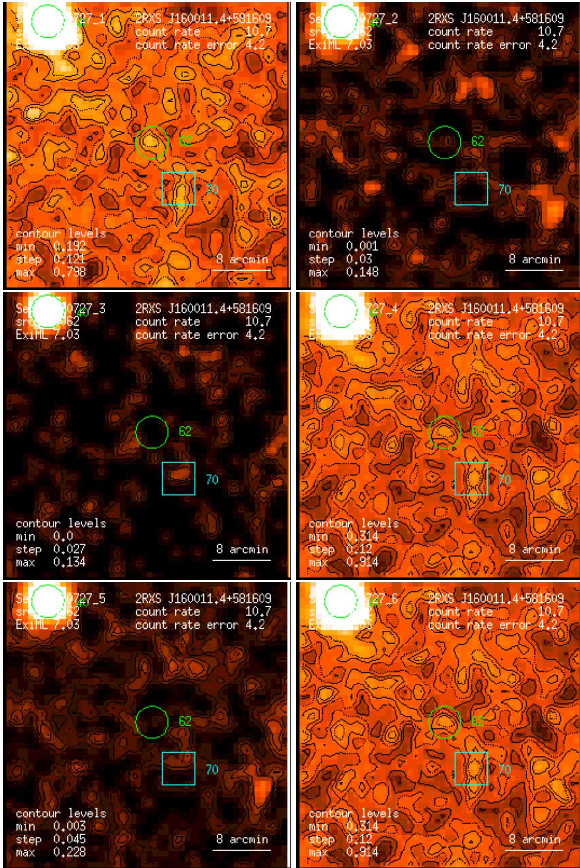
Figure 62: RASS 930727: detection 0062: band rate images, Gaussian filter: (1) PSPC channels 11 – 41, (2) 52 – 90, (3) 91 – 201, (4) 11 – 235, (5) 52 – 201, (6) 11 – 201. Broad band rates in counts/ks. Band rate contour levels in counts/ks/arcmin 2 .
