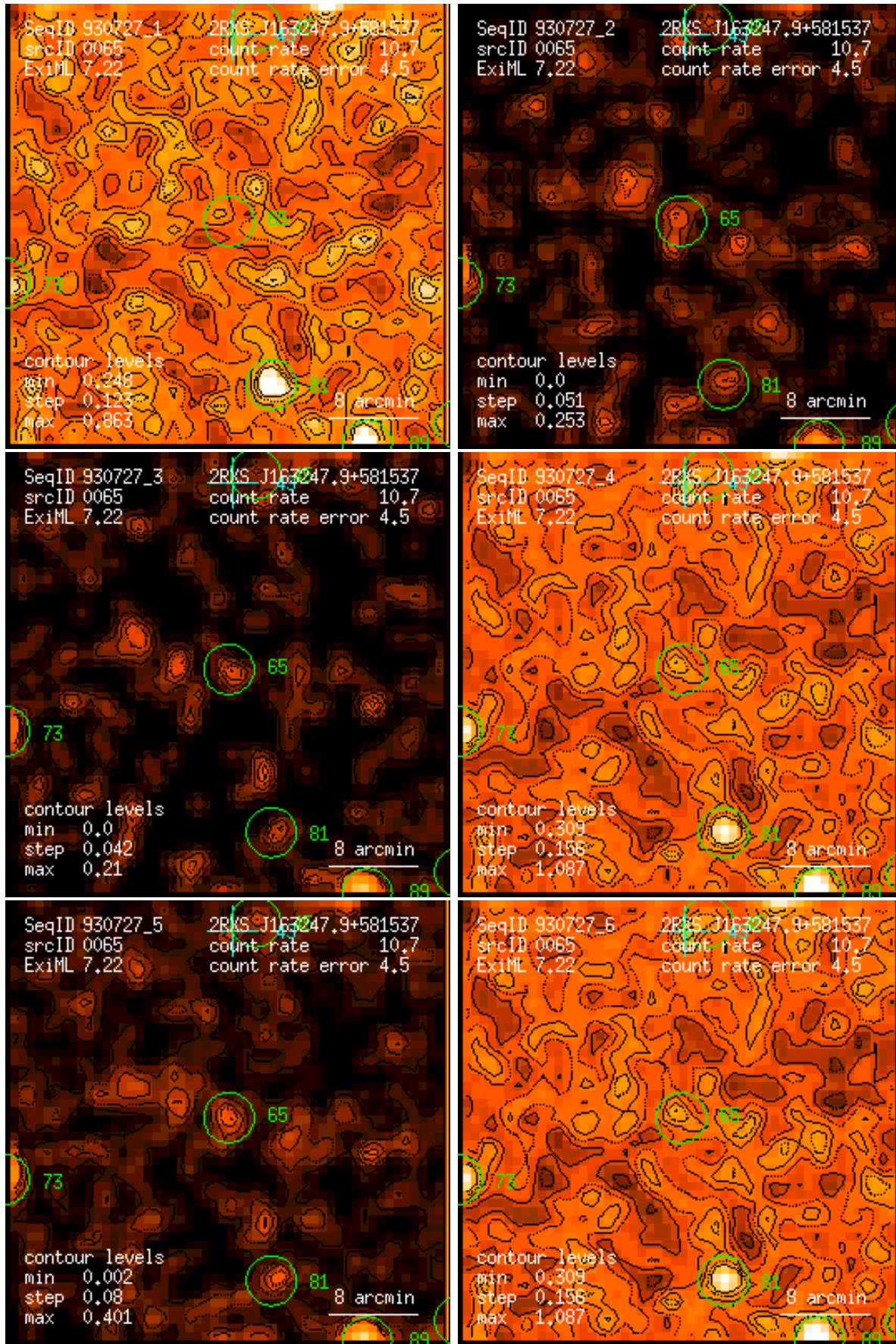
Figure 65: RASS 930727: detection 0065: band rate images, Gaussian filter: (1) PSPC channels 11 – 41, (2) 52 – 90, (3) 91 – 201, (4) 11 – 235, (5) 52 – 201, (6) 11 – 201. Broad band rates in counts/ks. Band rate contour levels in counts/ks/arcmin 2 .
