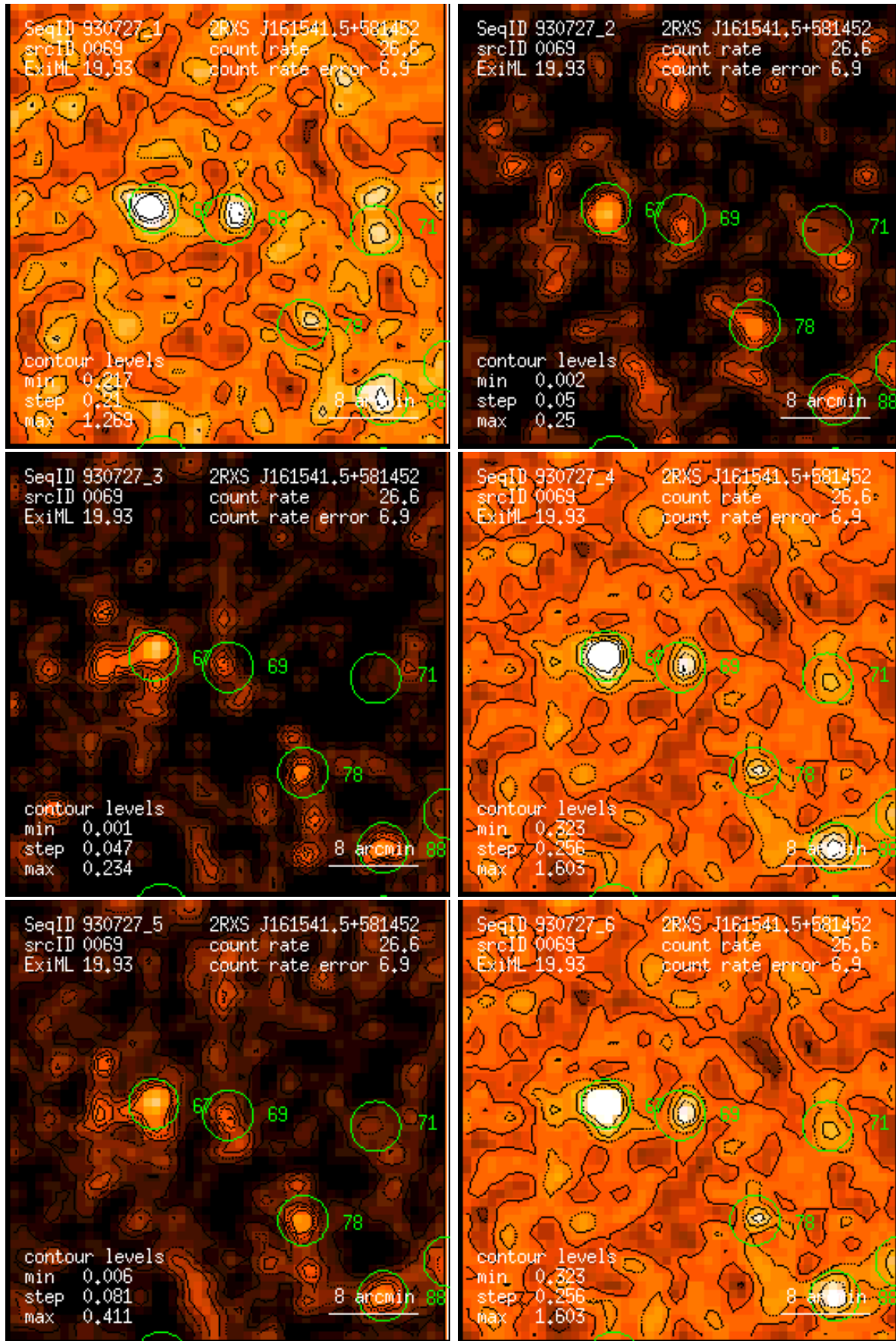
Figure 69: RASS 930727: detection 0069: band rate images, Gaussian filter: (1) PSPC channels 11 – 41, (2) 52 – 90, (3) 91 – 201, (4) 11 – 235, (5) 52 – 201, (6) 11 – 201. Broad band rates in counts/ks. Band rate contour levels in counts/ks/arcmin 2 .
