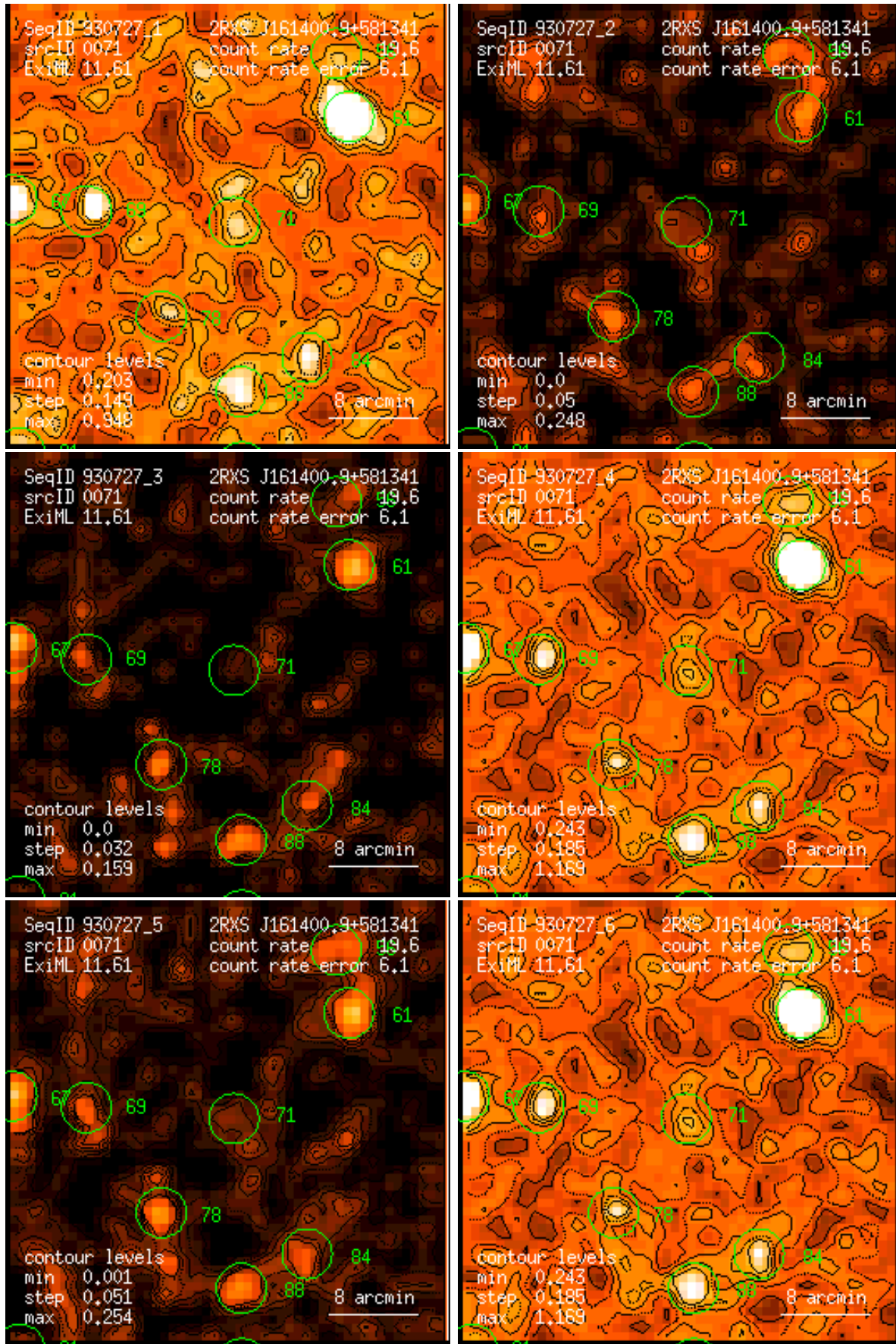
Figure 71: RASS 930727: detection 0071: band rate images, Gaussian filter: (1) PSPC channels 11 – 41, (2) 52 – 90, (3) 91 – 201, (4) 11 – 235, (5) 52 – 201, (6) 11 – 201. Broad band rates in counts/ks. Band rate contour levels in counts/ks/arcmin 2 .
