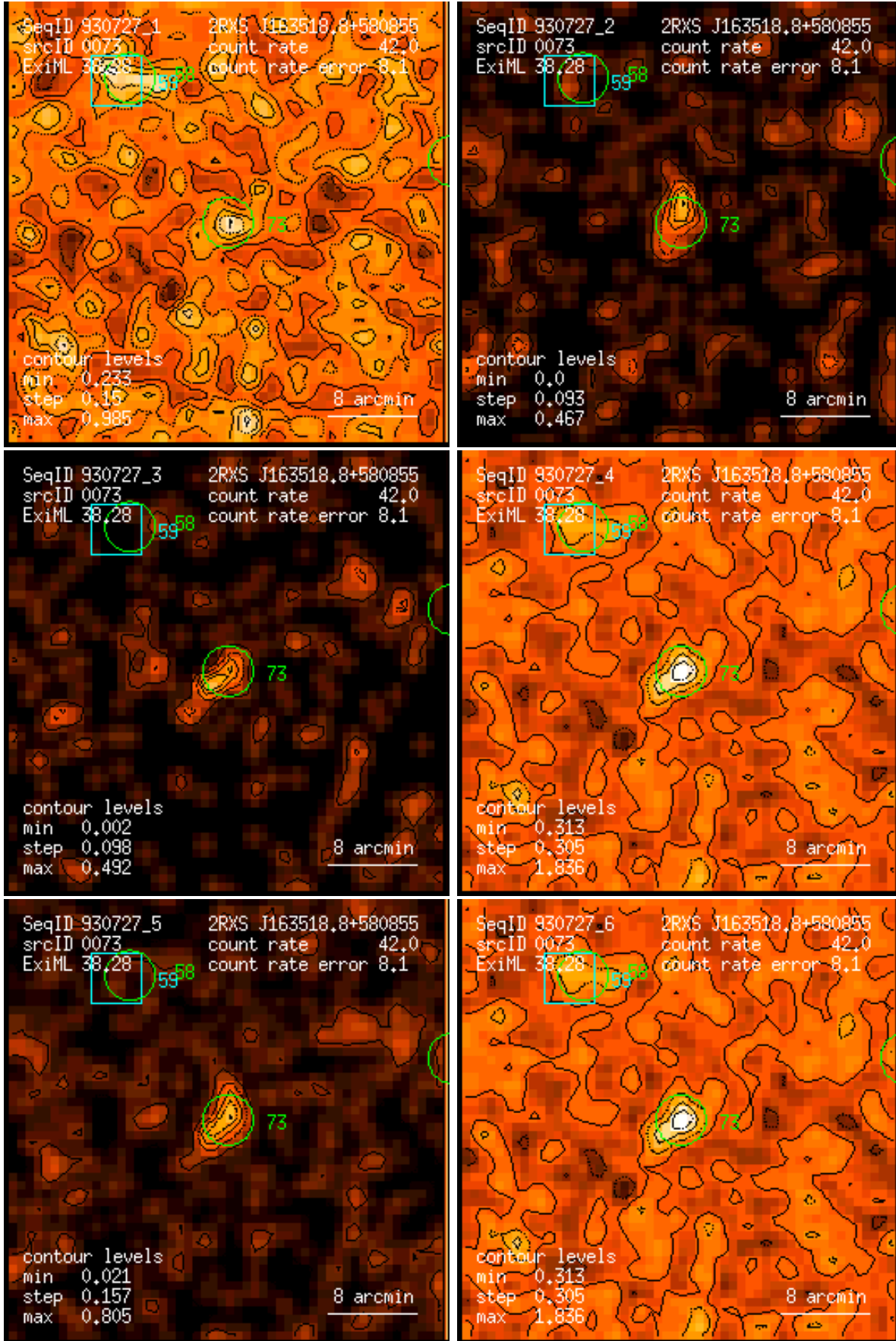
Figure 73: RASS 930727: detection 0073: band rate images, Gaussian filter: (1) PSPC channels 11 – 41, (2) 52 – 90, (3) 91 – 201, (4) 11 – 235, (5) 52 – 201, (6) 11 – 201. Broad band rates in counts/ks. Band rate contour levels in counts/ks/arcmin 2 .
