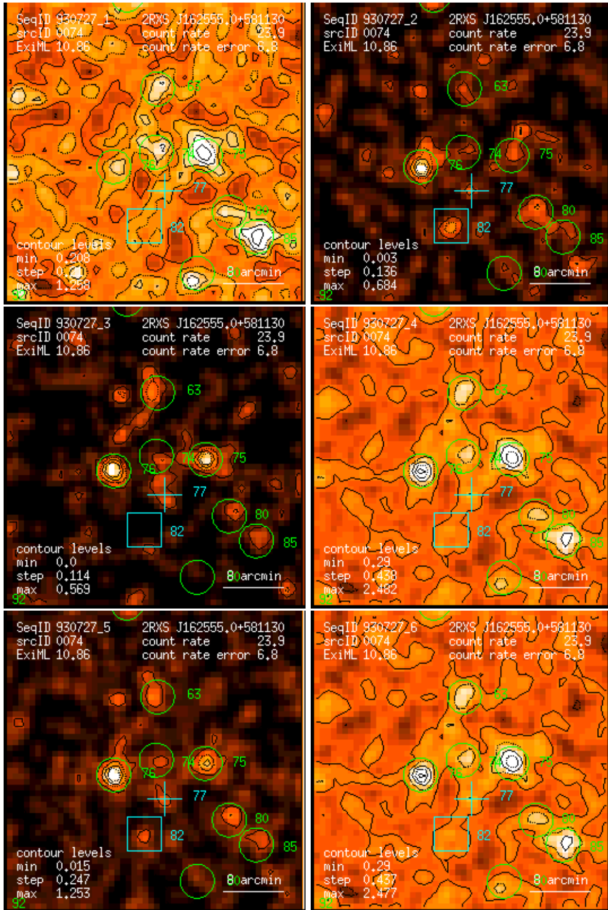
Figure 74: RASS 930727: detection 0074: band rate images, Gaussian filter: (1) PSPC channels 11 – 41, (2) 52 – 90, (3) 91 – 201, (4) 11 – 235, (5) 52 – 201, (6) 11 – 201. Broad band rates in counts/ks. Band rate contour levels in counts/ks/arcmin 2 .
