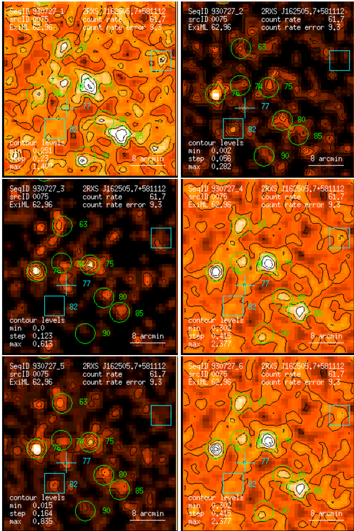
Figure 75: RASS 930727: detection 0075: band rate images, Gaussian filter: (1) PSPC channels 11 – 41, (2) 52 – 90, (3) 91 – 201, (4) 11 – 235, (5) 52 – 201, (6) 11 – 201. Broad band rates in counts/ks. Band rate contour levels in counts/ks/arcmin 2 .
