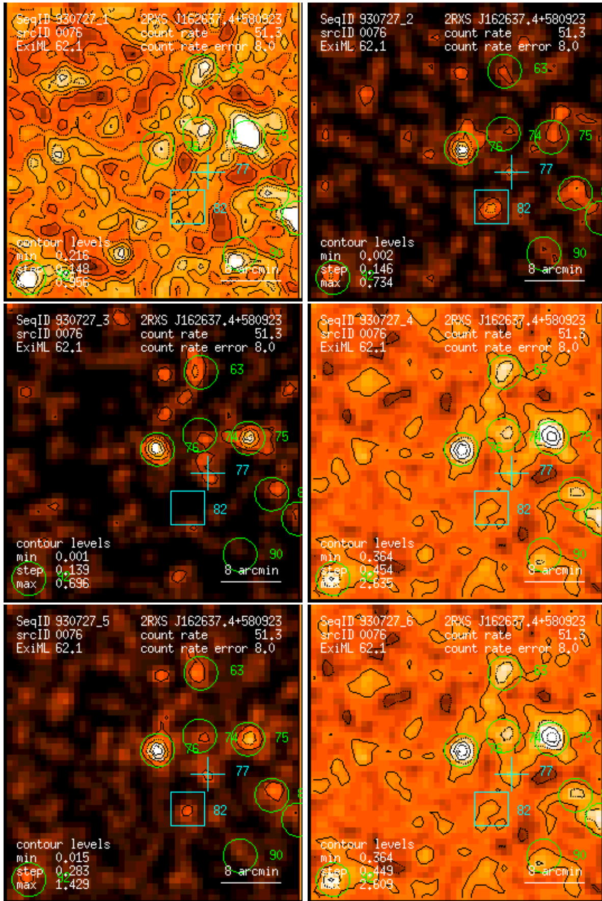
Figure 76: RASS 930727: detection 0076: band rate images, Gaussian filter: (1) PSPC channels 11 – 41, (2) 52 – 90, (3) 91 – 201, (4) 11 – 235, (5) 52 – 201, (6) 11 – 201. Broad band rates in counts/ks. Band rate contour levels in counts/ks/arcmin 2 .
