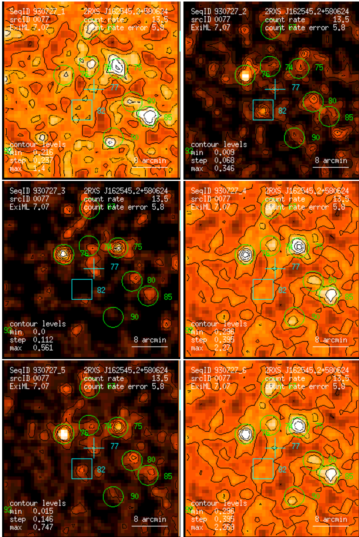
Figure 77: RASS 930727: detection 0077: band rate images, Gaussian filter: (1) PSPC channels 11 – 41, (2) 52 – 90, (3) 91 – 201, (4) 11 – 235, (5) 52 – 201, (6) 11 – 201. Broad band rates in counts/ks. Band rate contour levels in counts/ks/arcmin 2 .
