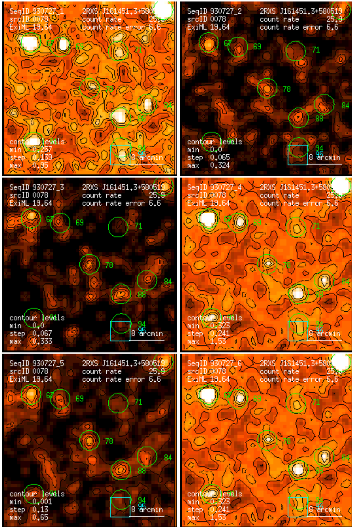
Figure 78: RASS 930727: detection 0078: band rate images, Gaussian filter: (1) PSPC channels 11 – 41, (2) 52 – 90, (3) 91 – 201, (4) 11 – 235, (5) 52 – 201, (6) 11 – 201. Broad band rates in counts/ks. Band rate contour levels in counts/ks/arcmin 2 .
