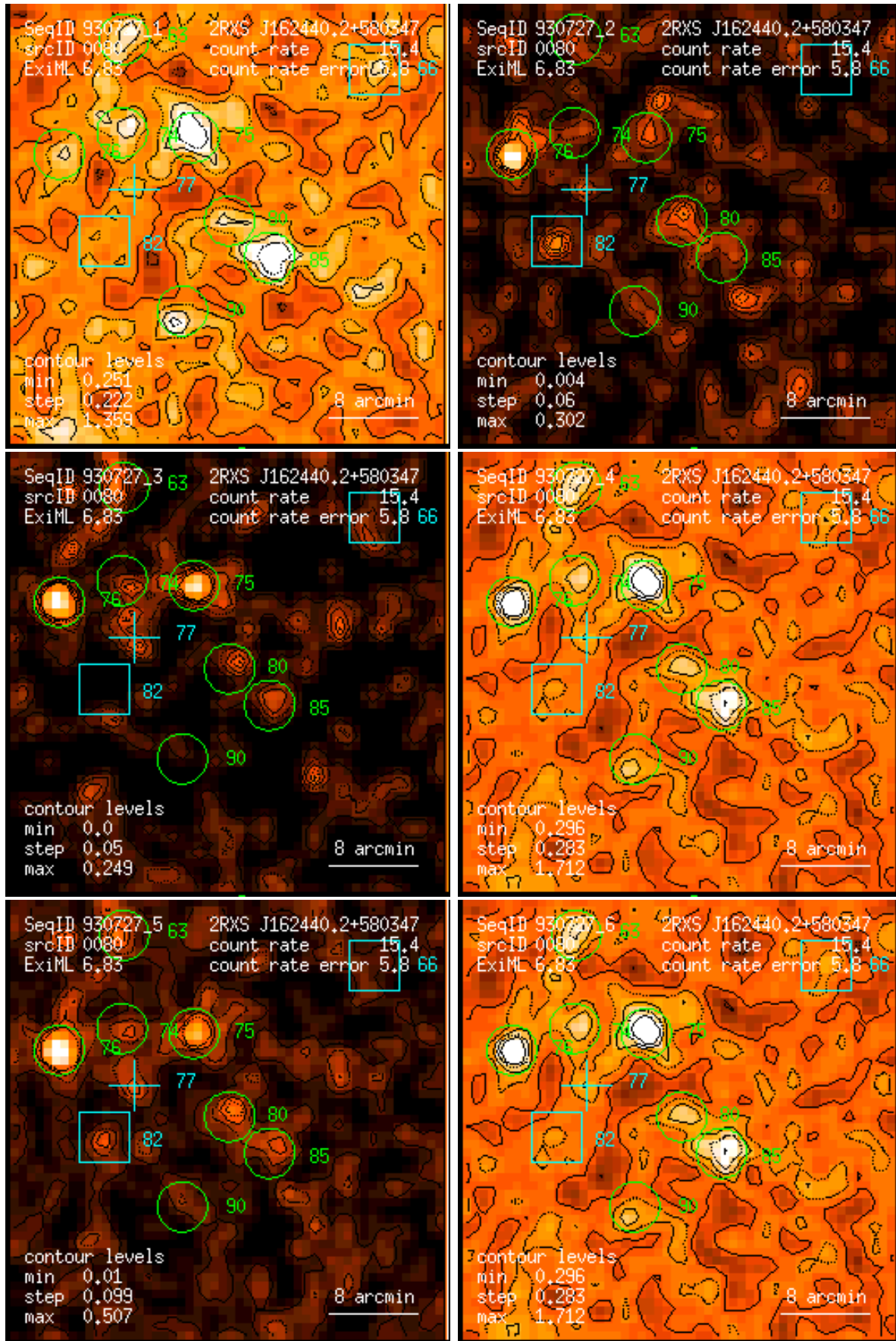
Figure 80: RASS 930727: detection 0080: band rate images, Gaussian filter: (1) PSPC channels 11 – 41, (2) 52 – 90, (3) 91 – 201, (4) 11 – 235, (5) 52 – 201, (6) 11 – 201. Broad band rates in counts/ks. Band rate contour levels in counts/ks/arcmin 2 .
