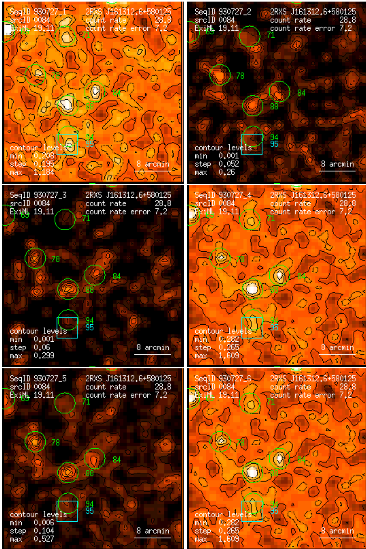
Figure 84: RASS 930727: detection 0084: band rate images, Gaussian filter: (1) PSPC channels 11 – 41, (2) 52 – 90, (3) 91 – 201, (4) 11 – 235, (5) 52 – 201, (6) 11 – 201. Broad band rates in counts/ks. Band rate contour levels in counts/ks/arcmin 2 .
