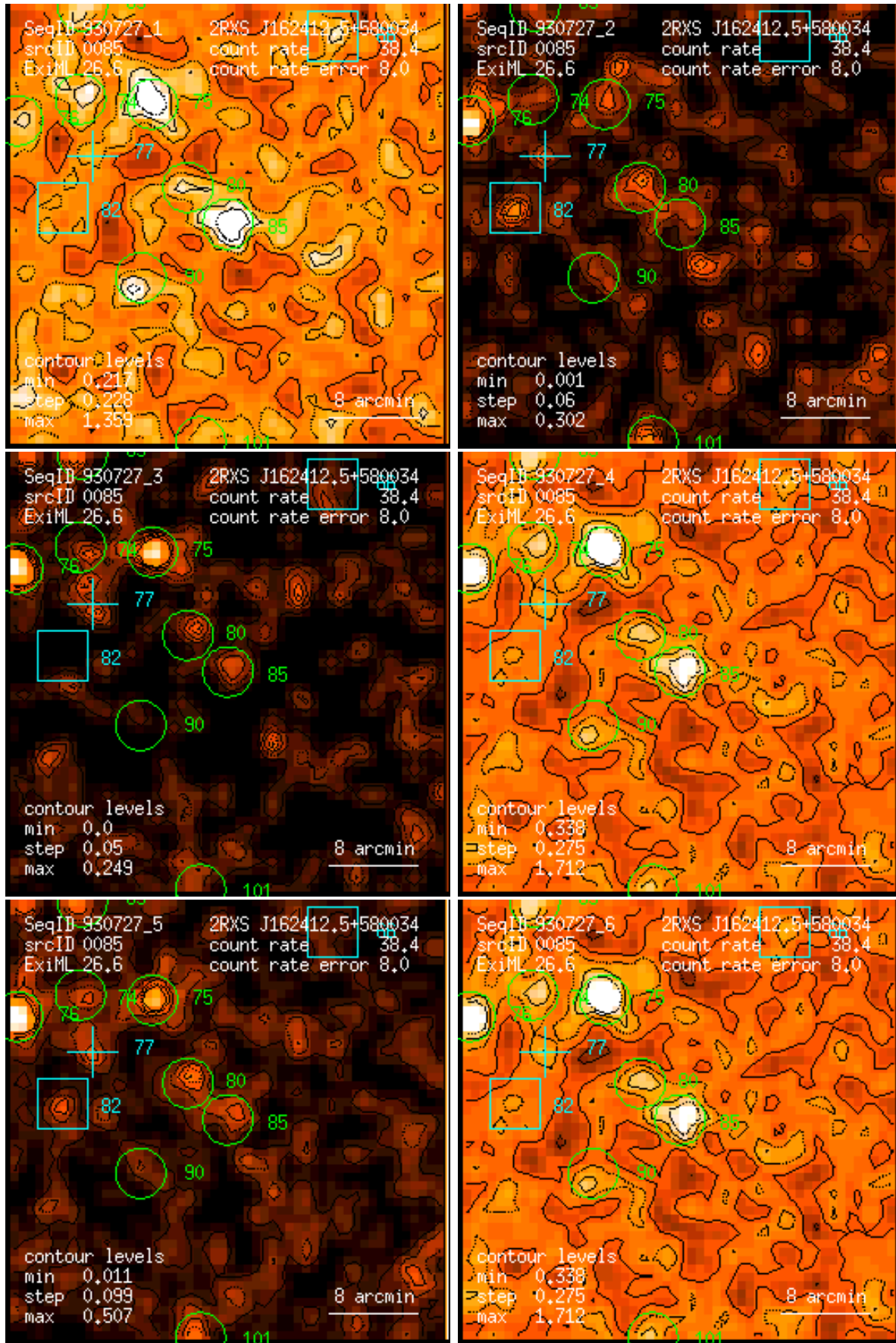
Figure 85: RASS 930727: detection 0085: band rate images, Gaussian filter: (1) PSPC channels 11 – 41, (2) 52 – 90, (3) 91 – 201, (4) 11 – 235, (5) 52 – 201, (6) 11 – 201. Broad band rates in counts/ks. Band rate contour levels in counts/ks/arcmin 2 .
