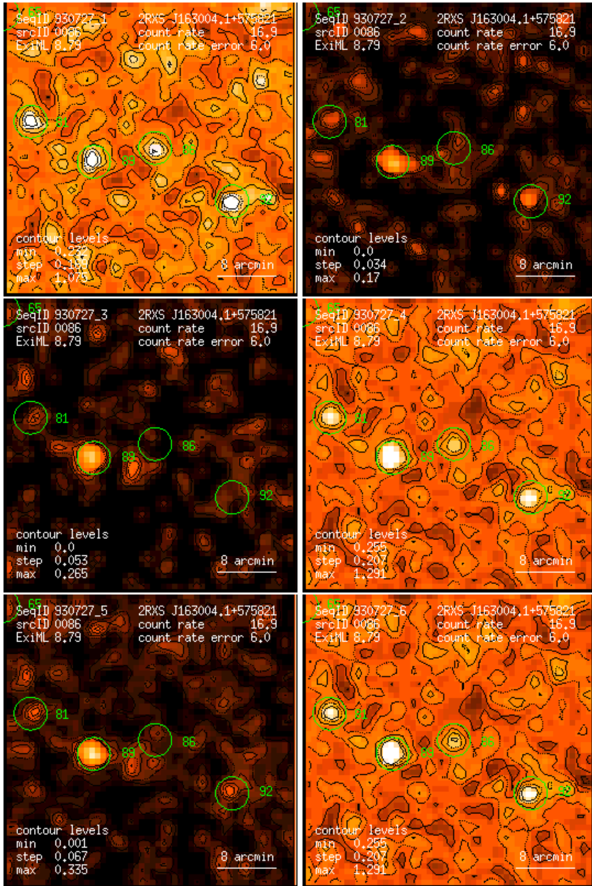
Figure 86: RASS 930727: detection 0086: band rate images, Gaussian filter: (1) PSPC channels 11 – 41, (2) 52 – 90, (3) 91 – 201, (4) 11 – 235, (5) 52 – 201, (6) 11 – 201. Broad band rates in counts/ks. Band rate contour levels in counts/ks/arcmin 2 .
