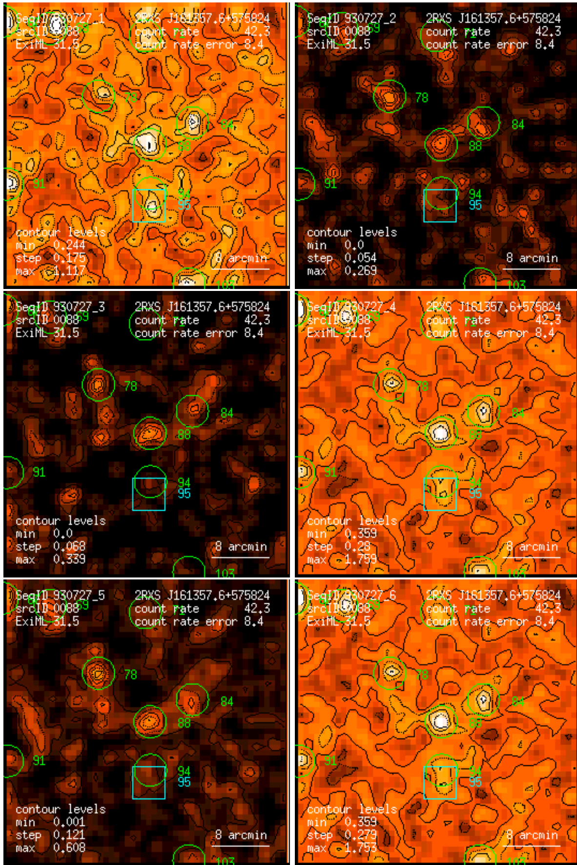
Figure 88: RASS 930727: detection 0088: band rate images, Gaussian filter: (1) PSPC channels 11 – 41, (2) 52 – 90, (3) 91 – 201, (4) 11 – 235, (5) 52 – 201, (6) 11 – 201. Broad band rates in counts/ks. Band rate contour levels in counts/ks/arcmin 2 .
