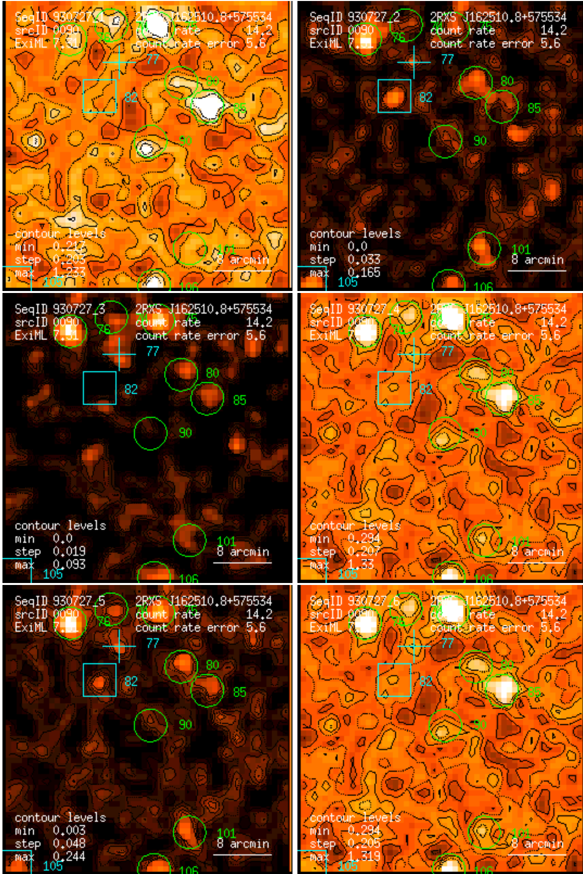
Figure 90: RASS 930727: detection 0090: band rate images, Gaussian filter: (1) PSPC channels 11 – 41, (2) 52 – 90, (3) 91 – 201, (4) 11 – 235, (5) 52 – 201, (6) 11 – 201. Broad band rates in counts/ks. Band rate contour levels in counts/ks/arcmin 2 .
