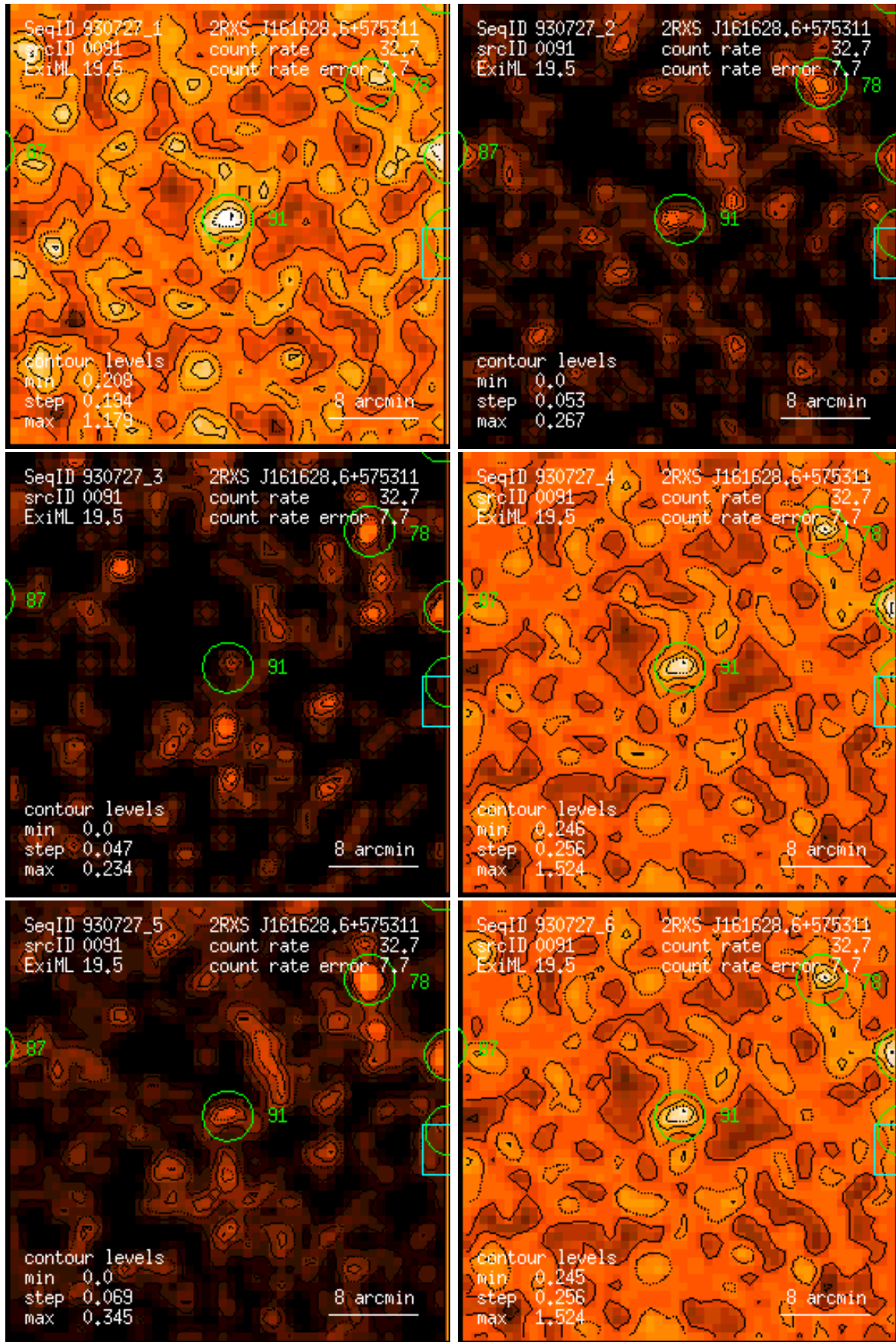
Figure 91: RASS 930727: detection 0091: band rate images, Gaussian filter: (1) PSPC channels 11 – 41, (2) 52 – 90, (3) 91 – 201, (4) 11 – 235, (5) 52 – 201, (6) 11 – 201. Broad band rates in counts/ks. Band rate contour levels in counts/ks/arcmin 2 .
