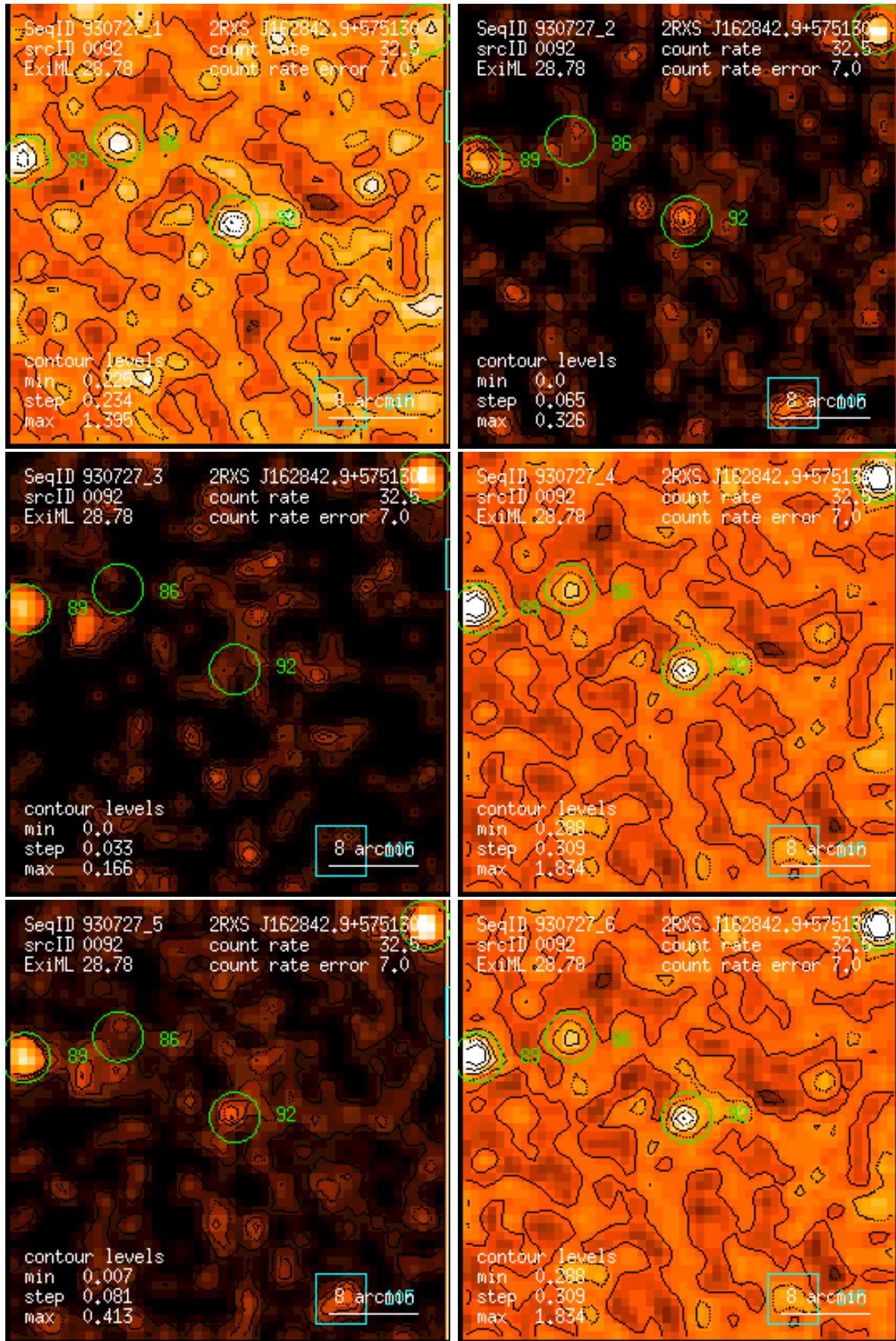
Figure 92: RASS 930727: detection 0092: band rate images, Gaussian filter: (1) PSPC channels 11 – 41, (2) 52 – 90, (3) 91 – 201, (4) 11 – 235, (5) 52 – 201, (6) 11 – 201. Broad band rates in counts/ks. Band rate contour levels in counts/ks/arcmin 2 .
