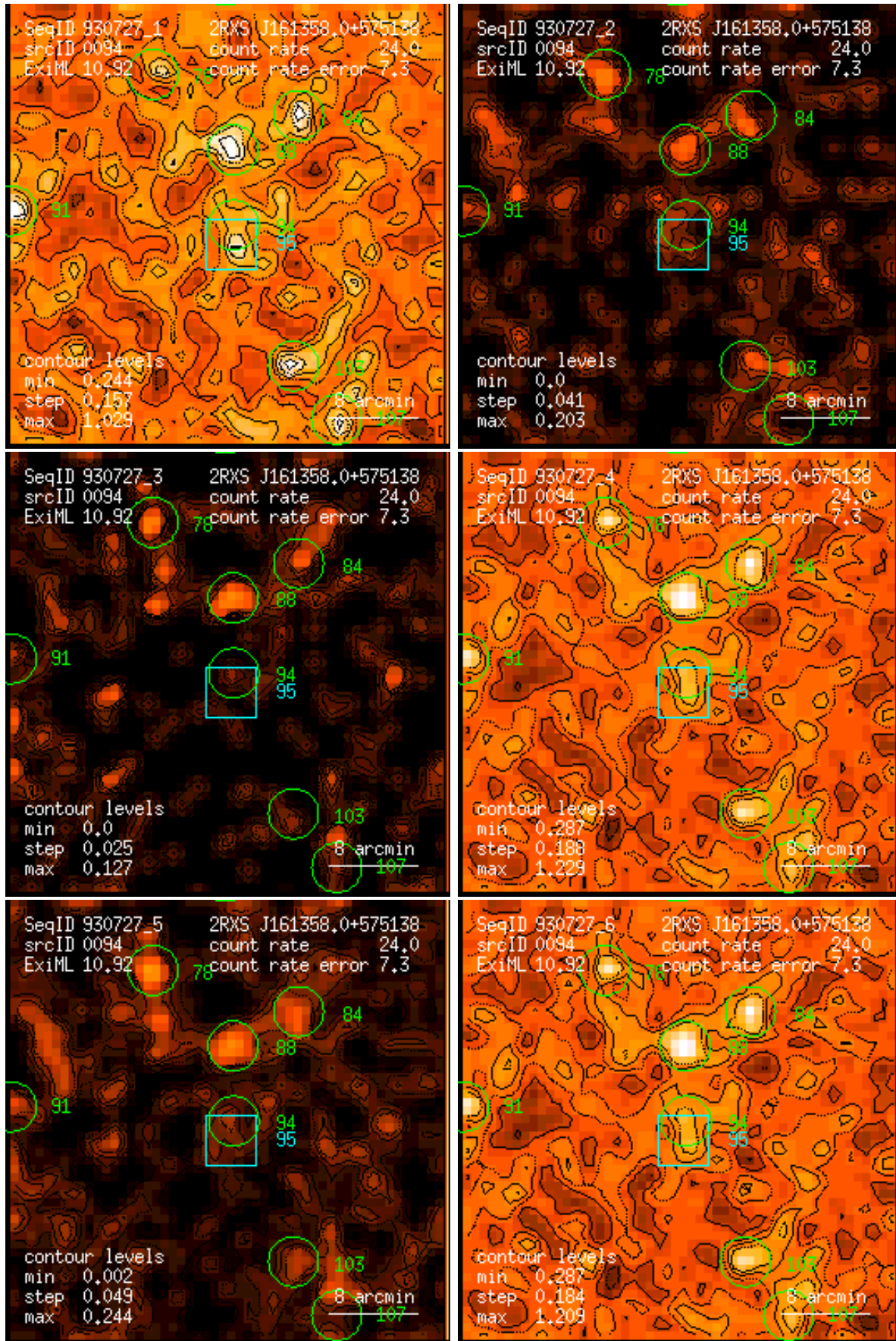
Figure 94: RASS 930727: detection 0094: band rate images, Gaussian filter: (1) PSPC channels 11 – 41, (2) 52 – 90, (3) 91 – 201, (4) 11 – 235, (5) 52 – 201, (6) 11 – 201. Broad band rates in counts/ks. Band rate contour levels in counts/ks/arcmin 2 .
