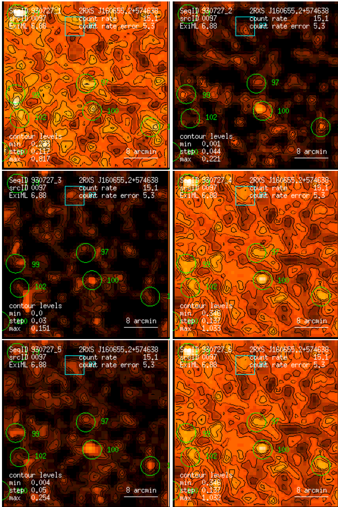
Figure 97: RASS 930727: detection 0097: band rate images, Gaussian filter: (1) PSPC channels 11 – 41, (2) 52 – 90, (3) 91 – 201, (4) 11 – 235, (5) 52 – 201, (6) 11 – 201. Broad band rates in counts/ks. Band rate contour levels in counts/ks/arcmin 2 .
