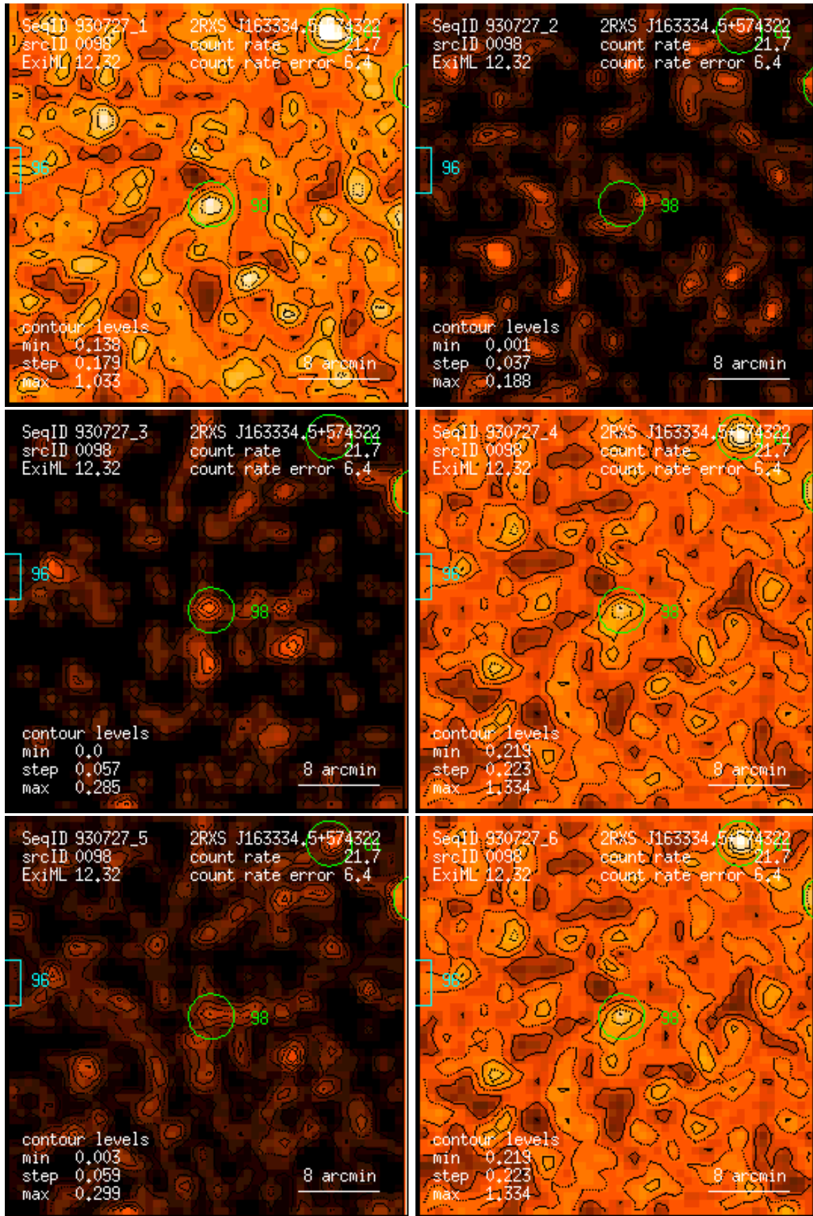
Figure 98: RASS 930727: detection 0098: band rate images, Gaussian filter: (1) PSPC channels 11 – 41, (2) 52 – 90, (3) 91 – 201, (4) 11 – 235, (5) 52 – 201, (6) 11 – 201. Broad band rates in counts/ks. Band rate contour levels in counts/ks/arcmin 2 .
