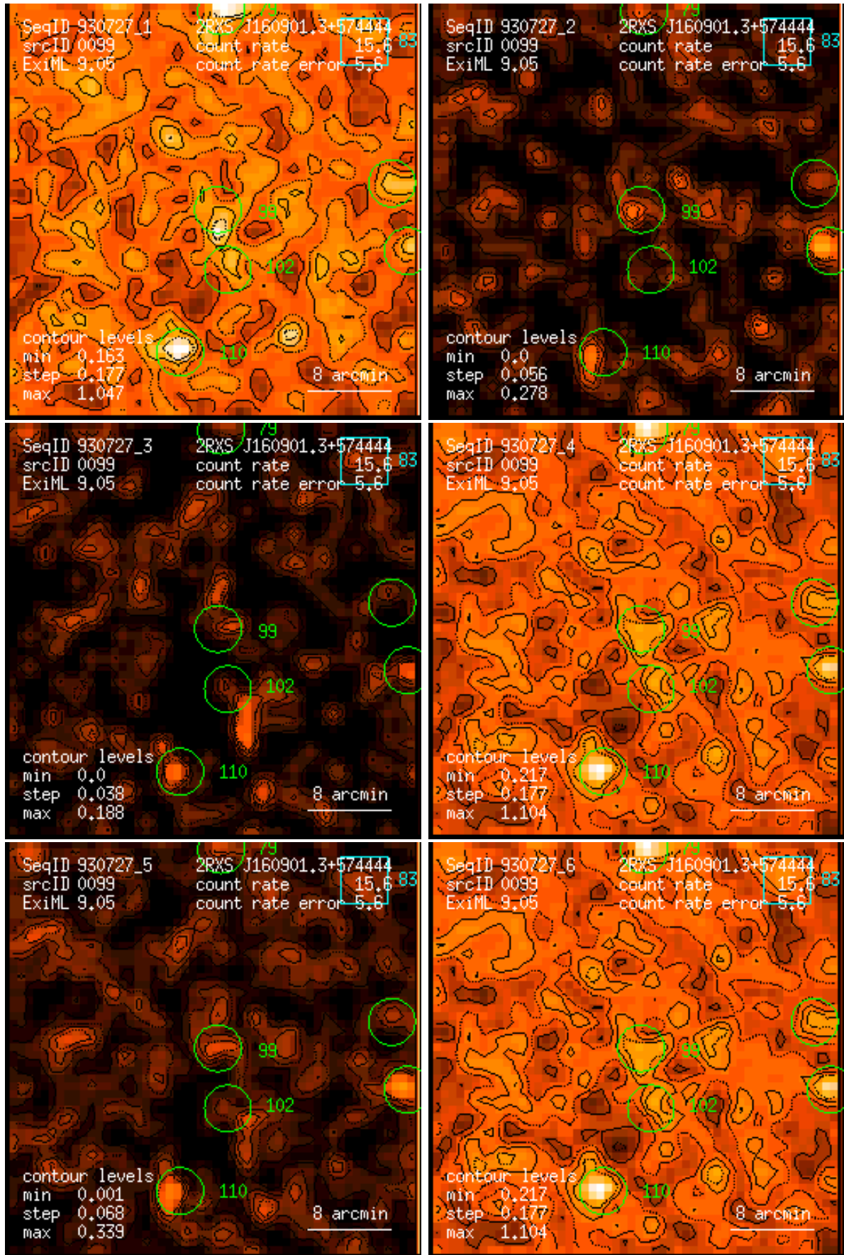
Figure 99: RASS 930727: detection 0099: band rate images, Gaussian filter: (1) PSPC channels 11 – 41, (2) 52 – 90, (3) 91 – 201, (4) 11 – 235, (5) 52 – 201, (6) 11 – 201. Broad band rates in counts/ks. Band rate contour levels in counts/ks/arcmin 2 .
