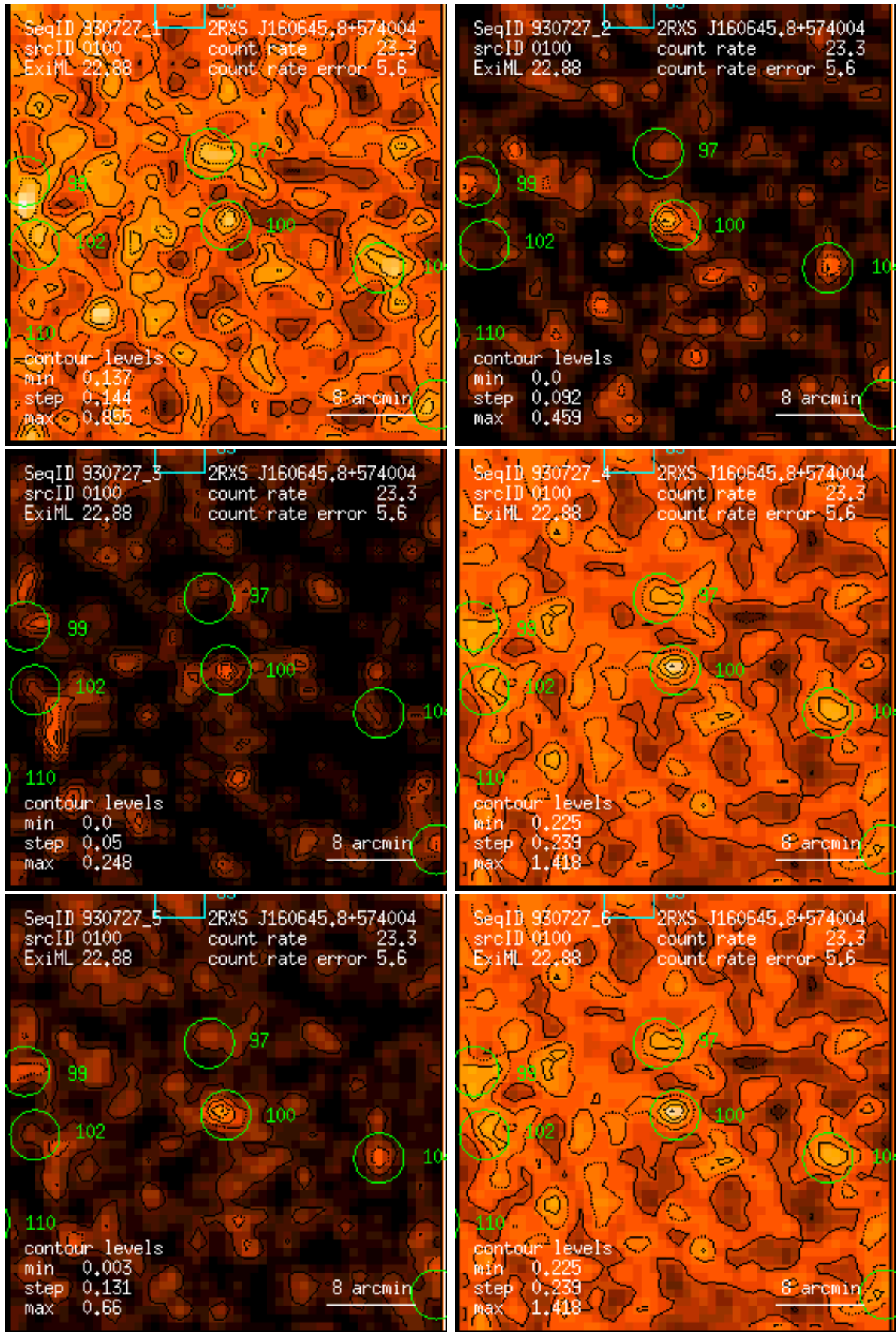
Figure 100: RASS 930727: detection 0100: band rate images, Gaussian filter: (1) PSPC channels 11 – 41, (2) 52 – 90, (3) 91 – 201, (4) 11 – 235, (5) 52 – 201, (6) 11 – 201. Broad band rates in counts/ks. Band rate contour levels in counts/ks/arcmin 2 .
