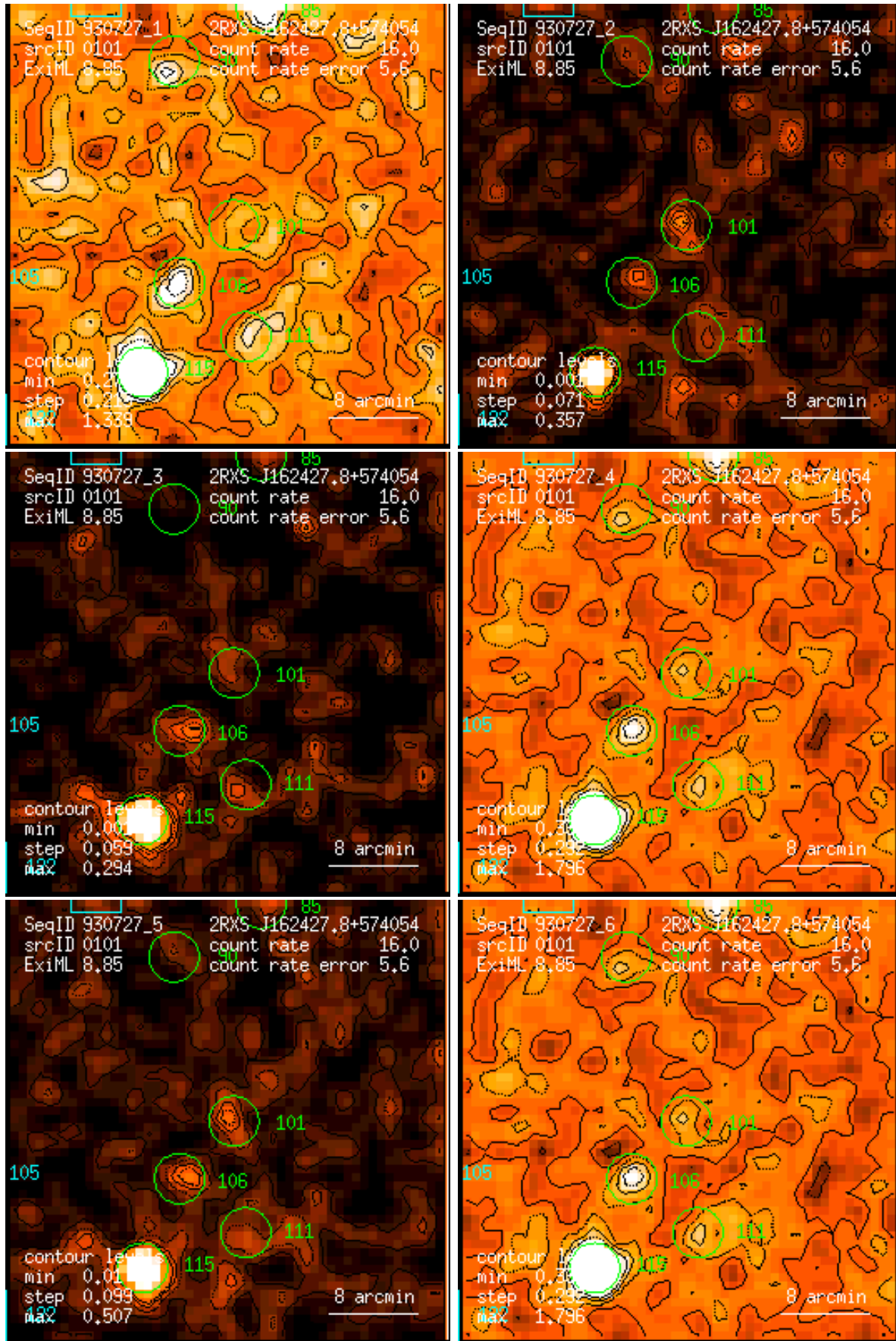
Figure 101: RASS 930727: detection 0101: band rate images, Gaussian filter: (1) PSPC channels 11 – 41, (2) 52 – 90, (3) 91 – 201, (4) 11 – 235, (5) 52 – 201, (6) 11 – 201. Broad band rates in counts/ks. Band rate contour levels in counts/ks/arcmin 2 .
