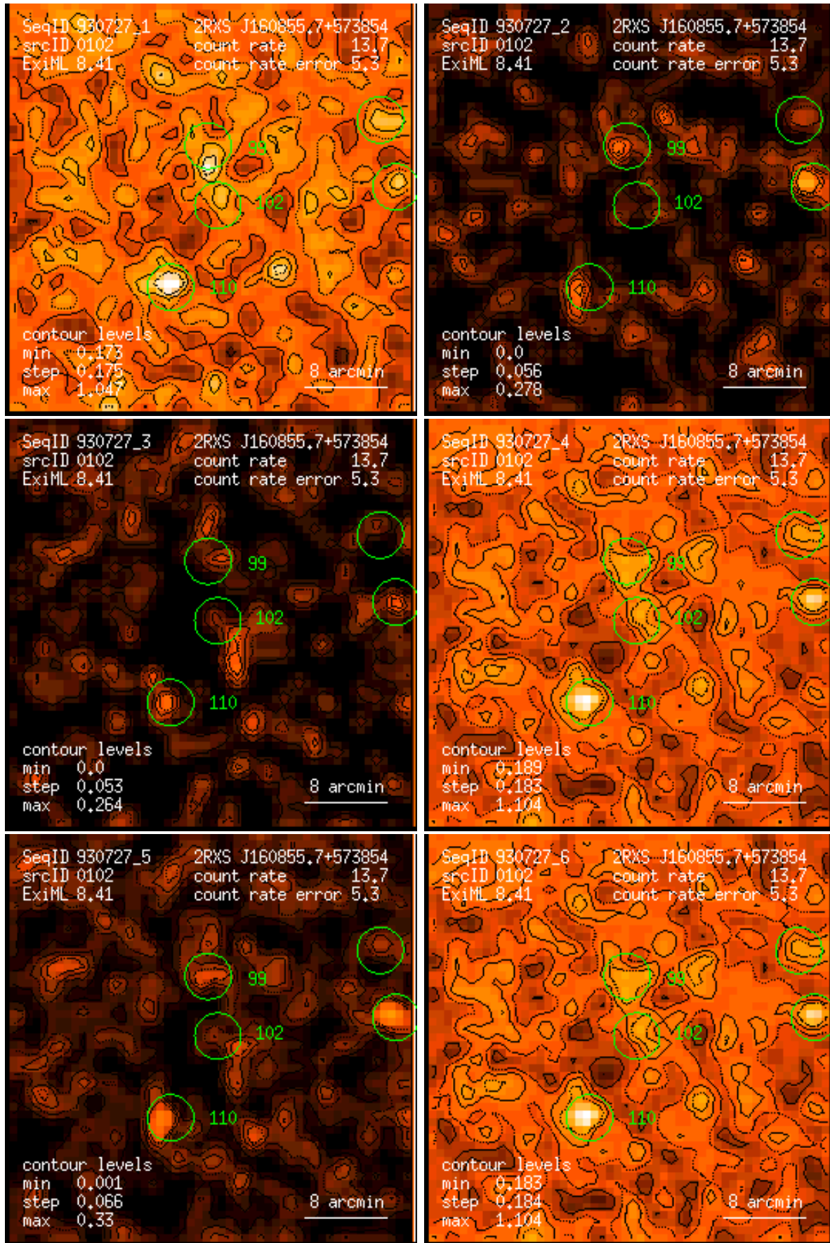
Figure 102: RASS 930727: detection 0102: band rate images, Gaussian filter: (1) PSPC channels 11 – 41, (2) 52 – 90, (3) 91 – 201, (4) 11 – 235, (5) 52 – 201, (6) 11 – 201. Broad band rates in counts/ks. Band rate contour levels in counts/ks/arcmin 2 .
