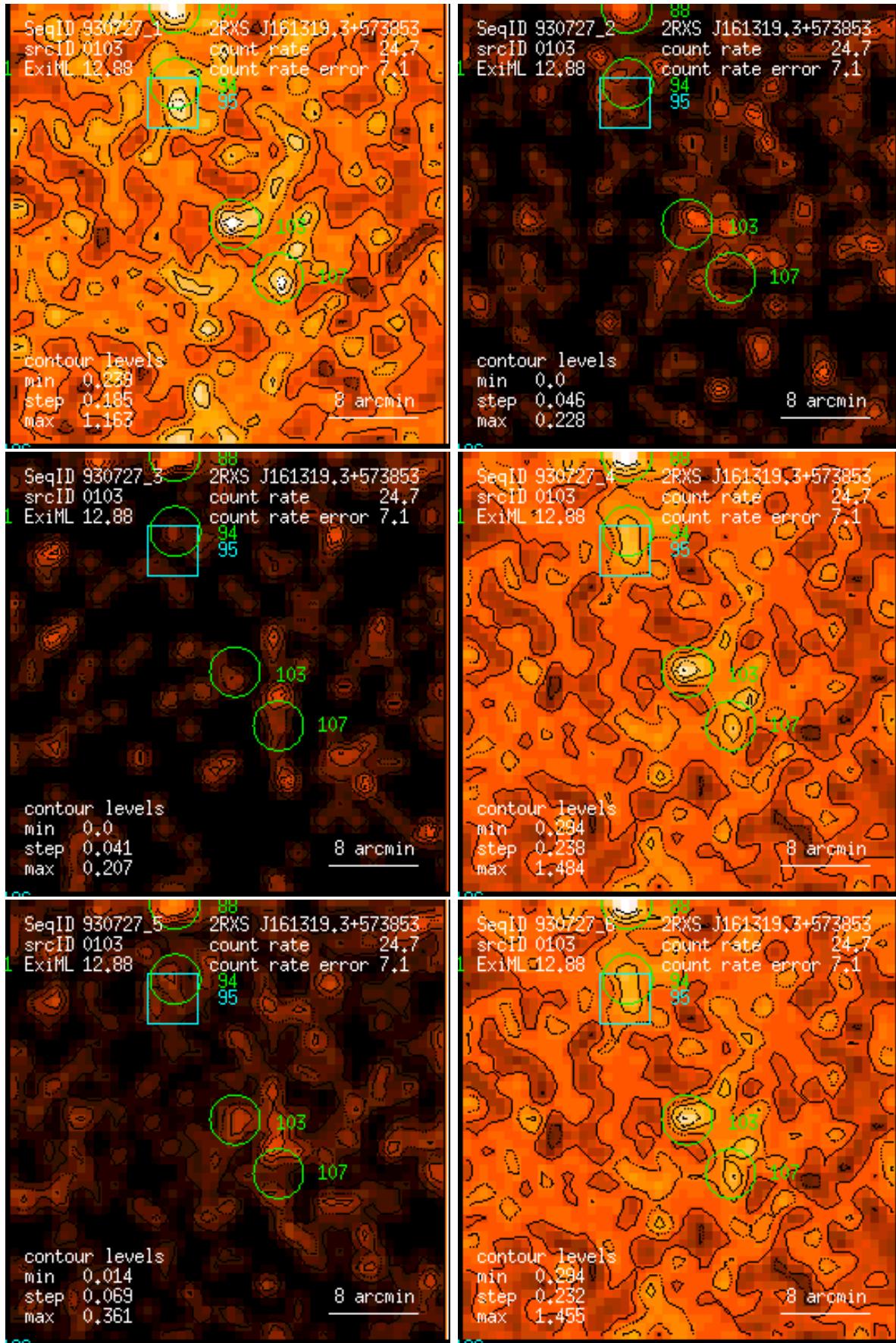
Figure 103: RASS 930727: detection 0103: band rate images, Gaussian filter: (1) PSPC channels 11 – 41, (2) 52 – 90, (3) 91 – 201, (4) 11 – 235, (5) 52 – 201, (6) 11 – 201. Broad band rates in counts/ks. Band rate contour levels in counts/ks/arcmin 2 .
