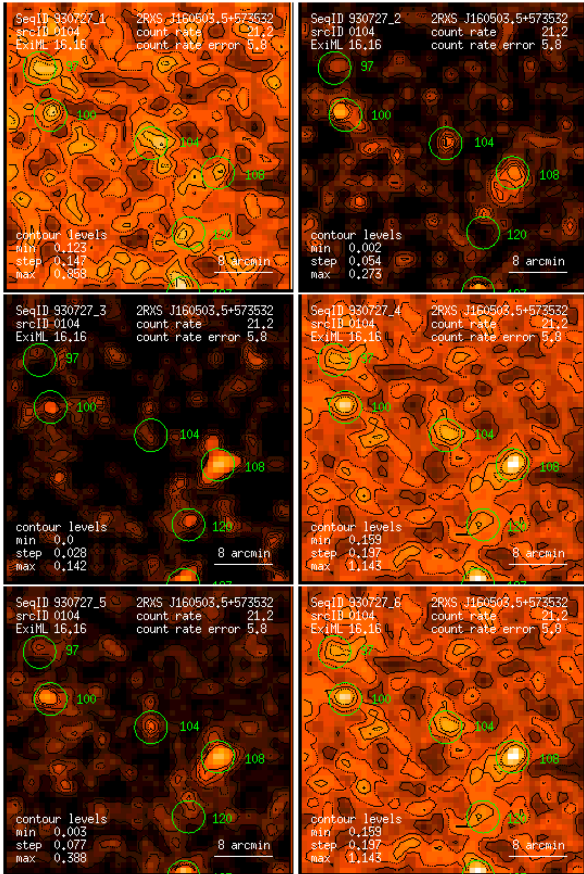
Figure 104: RASS 930727: detection 0104: band rate images, Gaussian filter: (1) PSPC channels 11 – 41, (2) 52 – 90, (3) 91 – 201, (4) 11 – 235, (5) 52 – 201, (6) 11 – 201. Broad band rates in counts/ks. Band rate contour levels in counts/ks/arcmin 2 .
